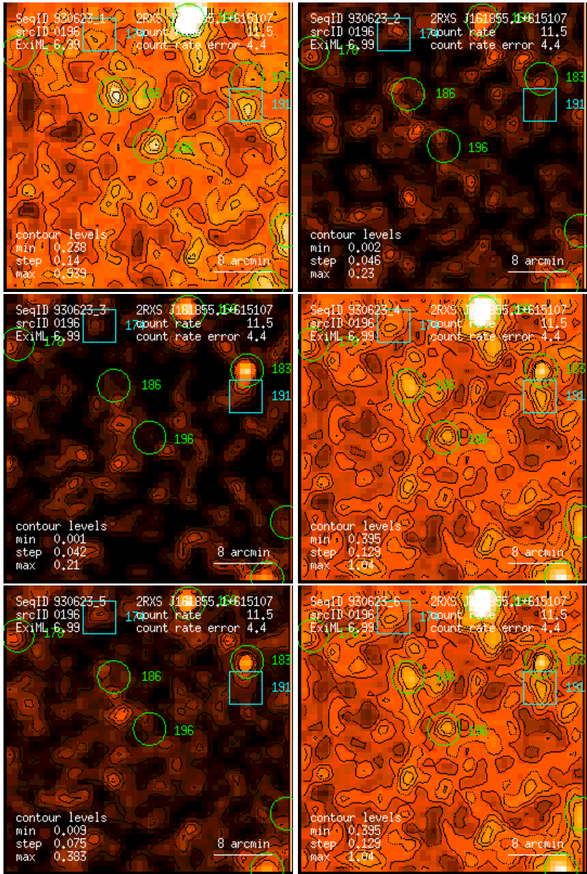
Figure 196: RASS 930623: detection 0196: band rate images, Gaussian filter: (1) PSPC channels 11 – 41, (2) 52 – 90, (3) 91 – 201, (4) 11 – 235, (5) 52 – 201, (6) 11 – 201. Broad band rates in counts/ks. Band rate contour levels in counts/ks/arcmin 2 .
