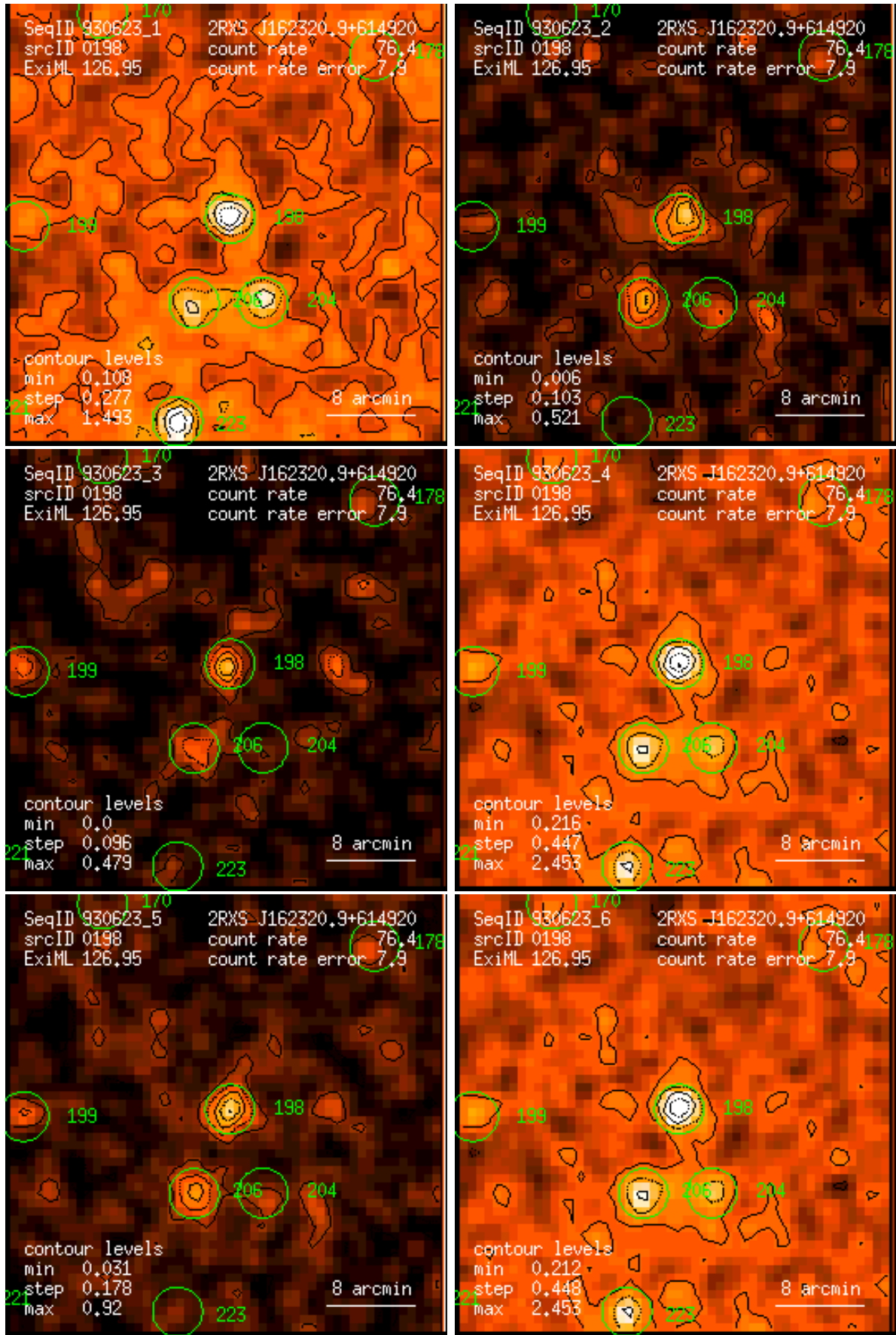
Figure 198: RASS 930623: detection 0198: band rate images, Gaussian filter: (1) PSPC channels 11 – 41, (2) 52 – 90, (3) 91 – 201, (4) 11 – 235, (5) 52 – 201, (6) 11 – 201. Broad band rates in counts/ks. Band rate contour levels in counts/ks/arcmin 2 .
