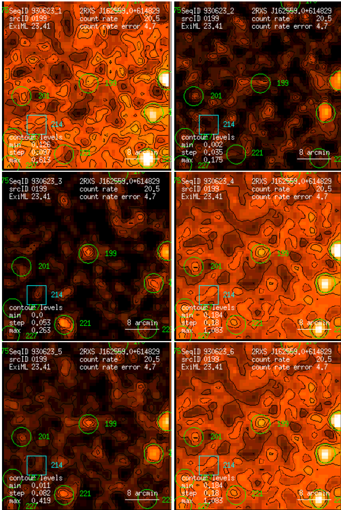
Figure 199: RASS 930623: detection 0199: band rate images, Gaussian filter: (1) PSPC channels 11 – 41, (2) 52 – 90, (3) 91 – 201, (4) 11 – 235, (5) 52 – 201, (6) 11 – 201. Broad band rates in counts/ks. Band rate contour levels in counts/ks/arcmin 2 .
