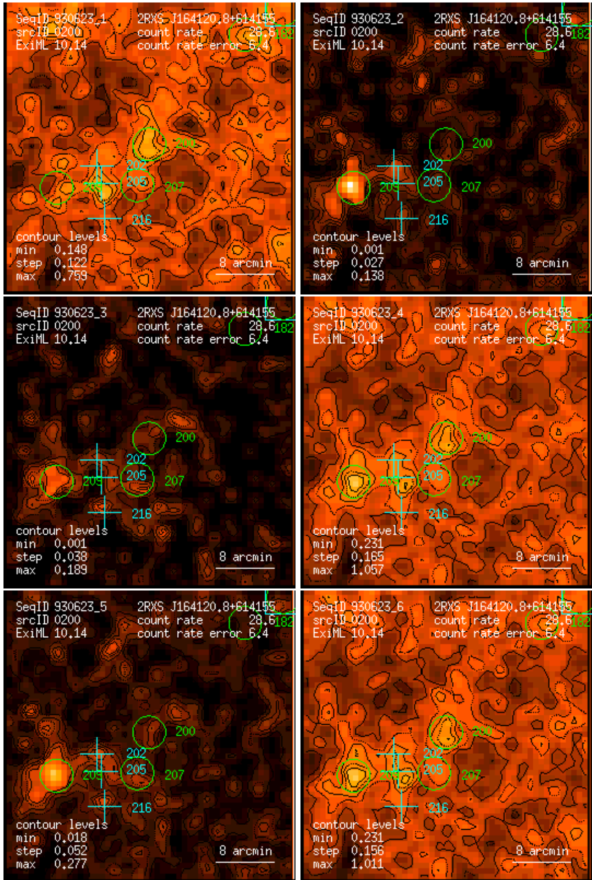
Figure 200: RASS 930623: detection 0200: band rate images, Gaussian filter: (1) PSPC channels 11 – 41, (2) 52 – 90, (3) 91 – 201, (4) 11 – 235, (5) 52 – 201, (6) 11 – 201. Broad band rates in counts/ks. Band rate contour levels in counts/ks/arcmin 2 .
