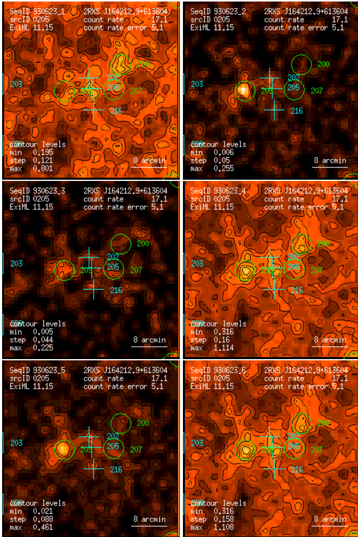
Figure 205: RASS 930623: detection 0205: band rate images, Gaussian filter: (1) PSPC channels 11 – 41, (2) 52 – 90, (3) 91 – 201, (4) 11 – 235, (5) 52 – 201, (6) 11 – 201. Broad band rates in counts/ks. Band rate contour levels in counts/ks/arcmin 2 .
