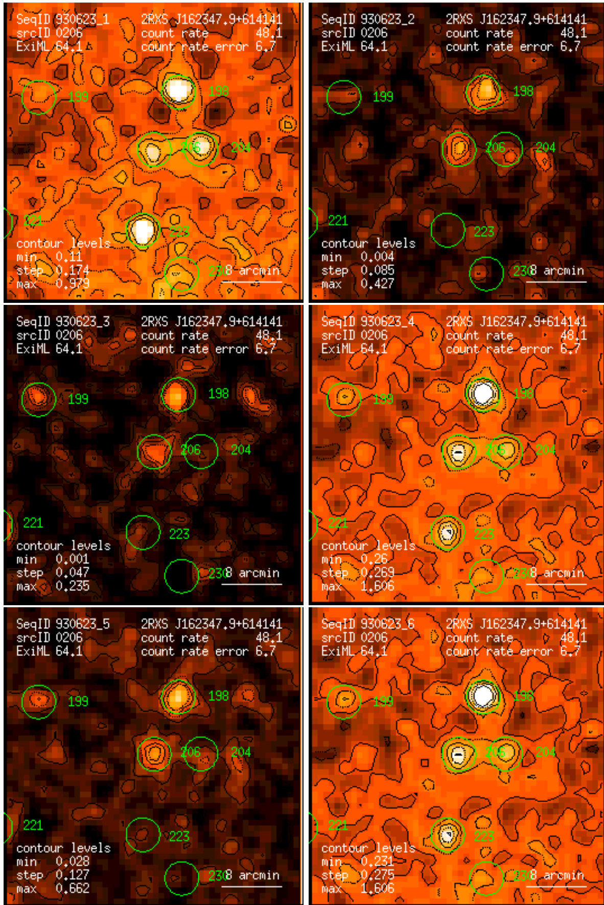
Figure 206: RASS 930623: detection 0206: band rate images, Gaussian filter: (1) PSPC channels 11 – 41, (2) 52 – 90, (3) 91 – 201, (4) 11 – 235, (5) 52 – 201, (6) 11 – 201. Broad band rates in counts/ks. Band rate contour levels in counts/ks/arcmin 2 .
