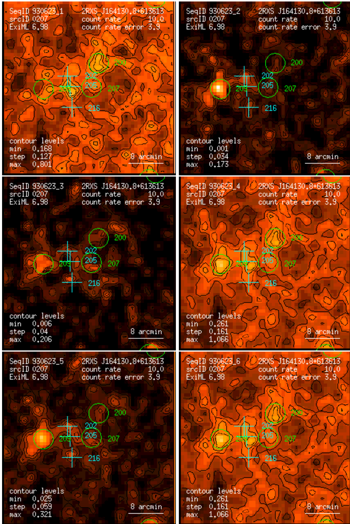
Figure 207: RASS 930623: detection 0207: band rate images, Gaussian filter: (1) PSPC channels 11 – 41, (2) 52 – 90, (3) 91 – 201, (4) 11 – 235, (5) 52 – 201, (6) 11 – 201. Broad band rates in counts/ks. Band rate contour levels in counts/ks/arcmin 2 .
