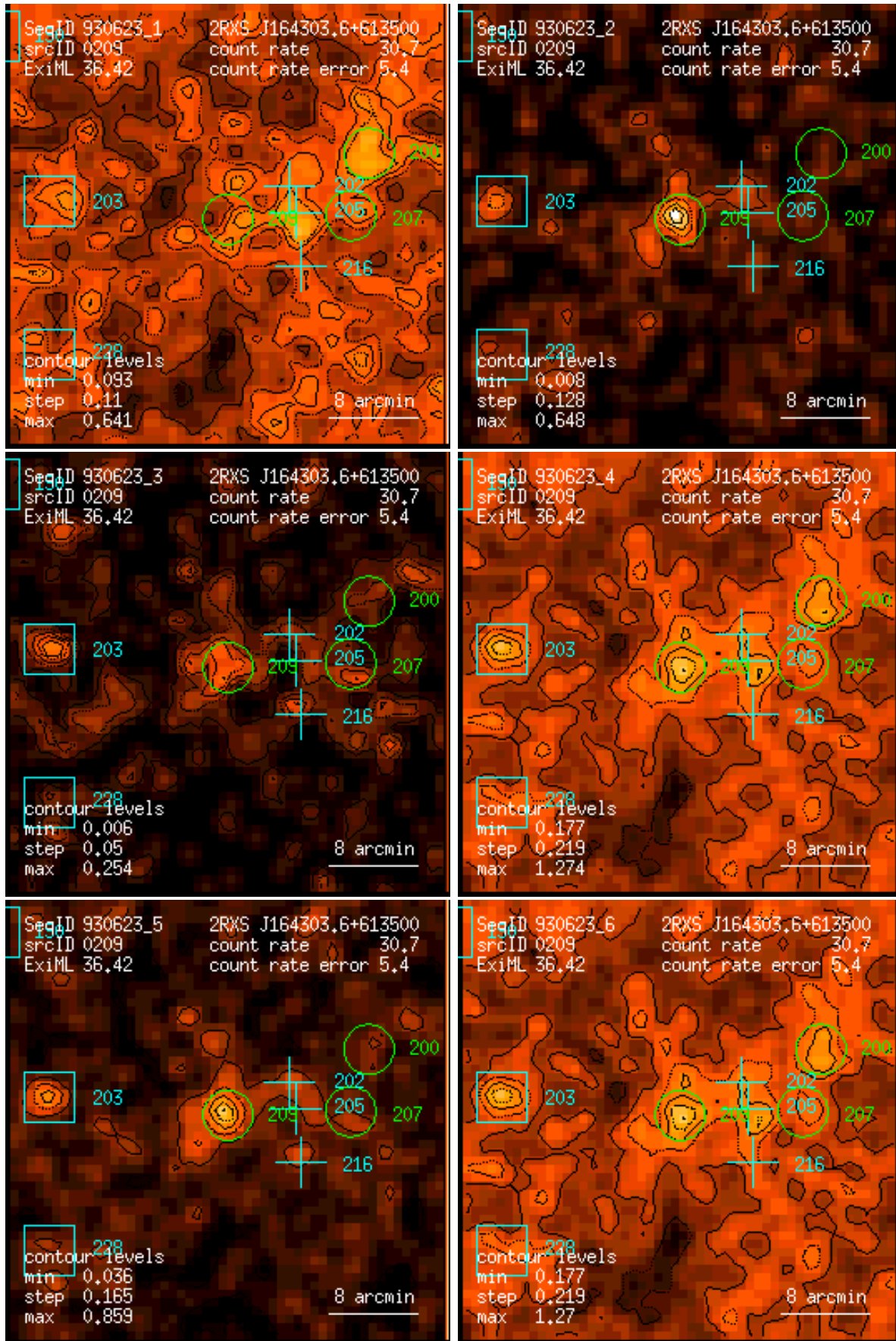
Figure 209: RASS 930623: detection 0209: band rate images, Gaussian filter: (1) PSPC channels 11 – 41, (2) 52 – 90, (3) 91 – 201, (4) 11 – 235, (5) 52 – 201, (6) 11 – 201. Broad band rates in counts/ks. Band rate contour levels in counts/ks/arcmin 2 .
