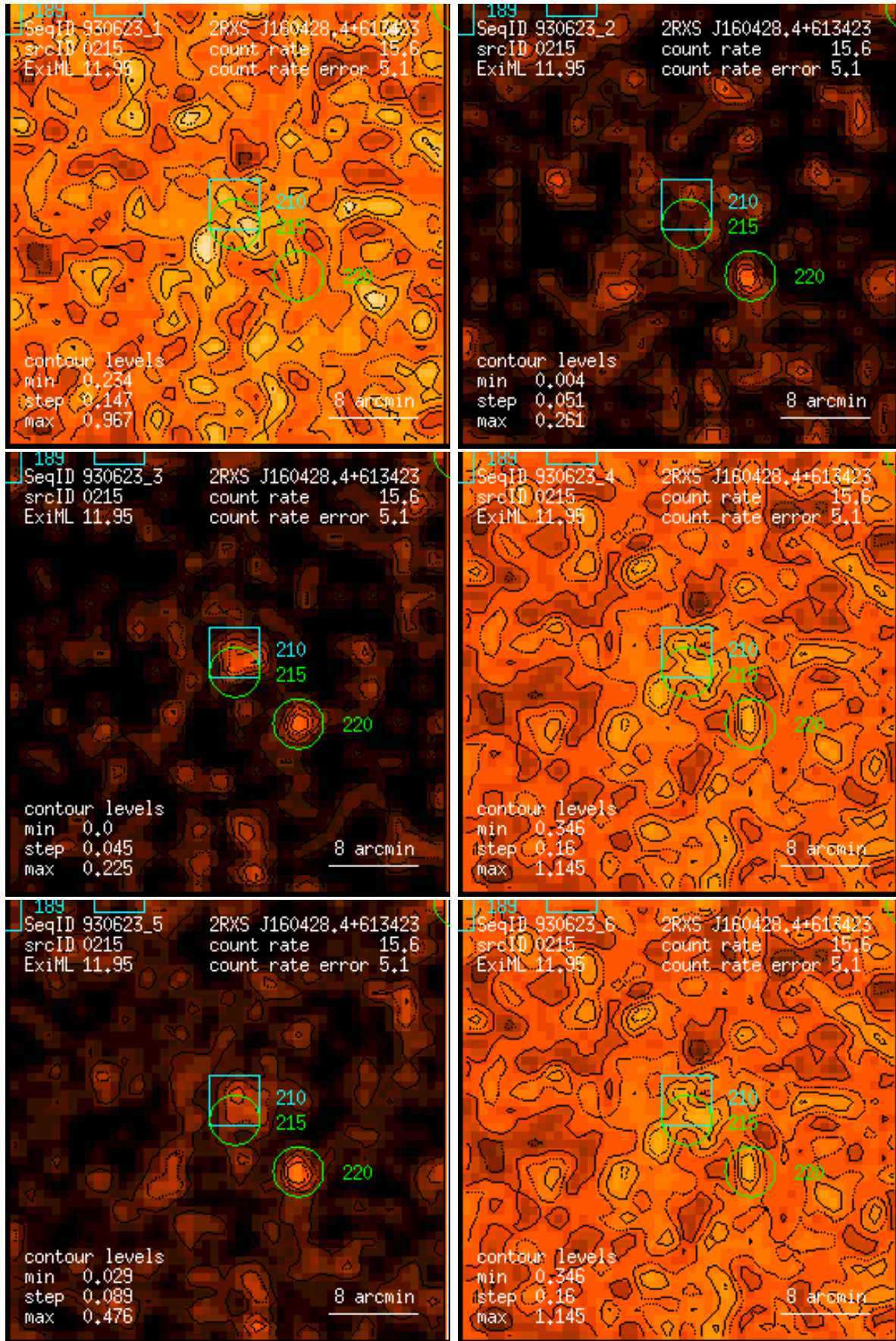
Figure 215: RASS 930623: detection 0215: band rate images, Gaussian filter: (1) PSPC channels 11 – 41, (2) 52 – 90, (3) 91 – 201, (4) 11 – 235, (5) 52 – 201, (6) 11 – 201. Broad band rates in counts/ks. Band rate contour levels in counts/ks/arcmin 2 .
