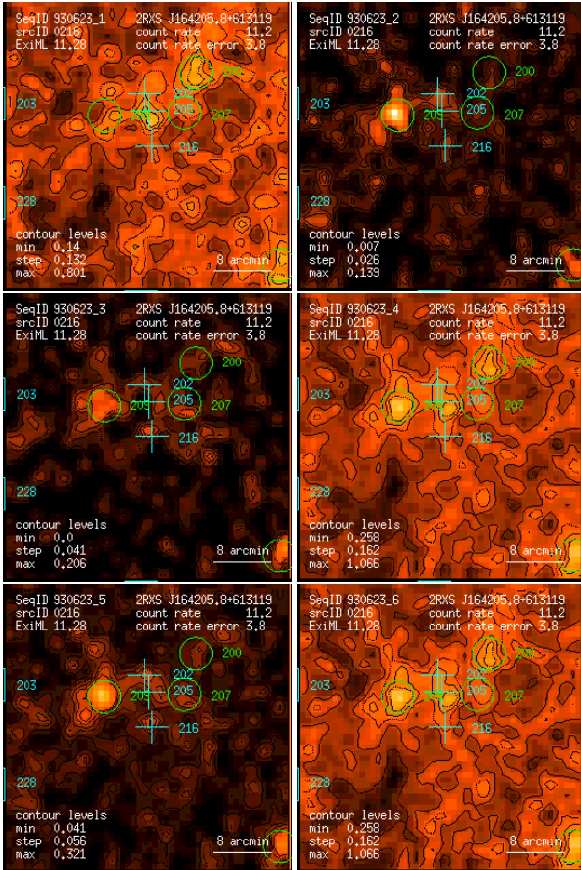
Figure 216: RASS 930623: detection 0216: band rate images, Gaussian filter: (1) PSPC channels 11 – 41, (2) 52 – 90, (3) 91 – 201, (4) 11 – 235, (5) 52 – 201, (6) 11 – 201. Broad band rates in counts/ks. Band rate contour levels in counts/ks/arcmin 2 .
