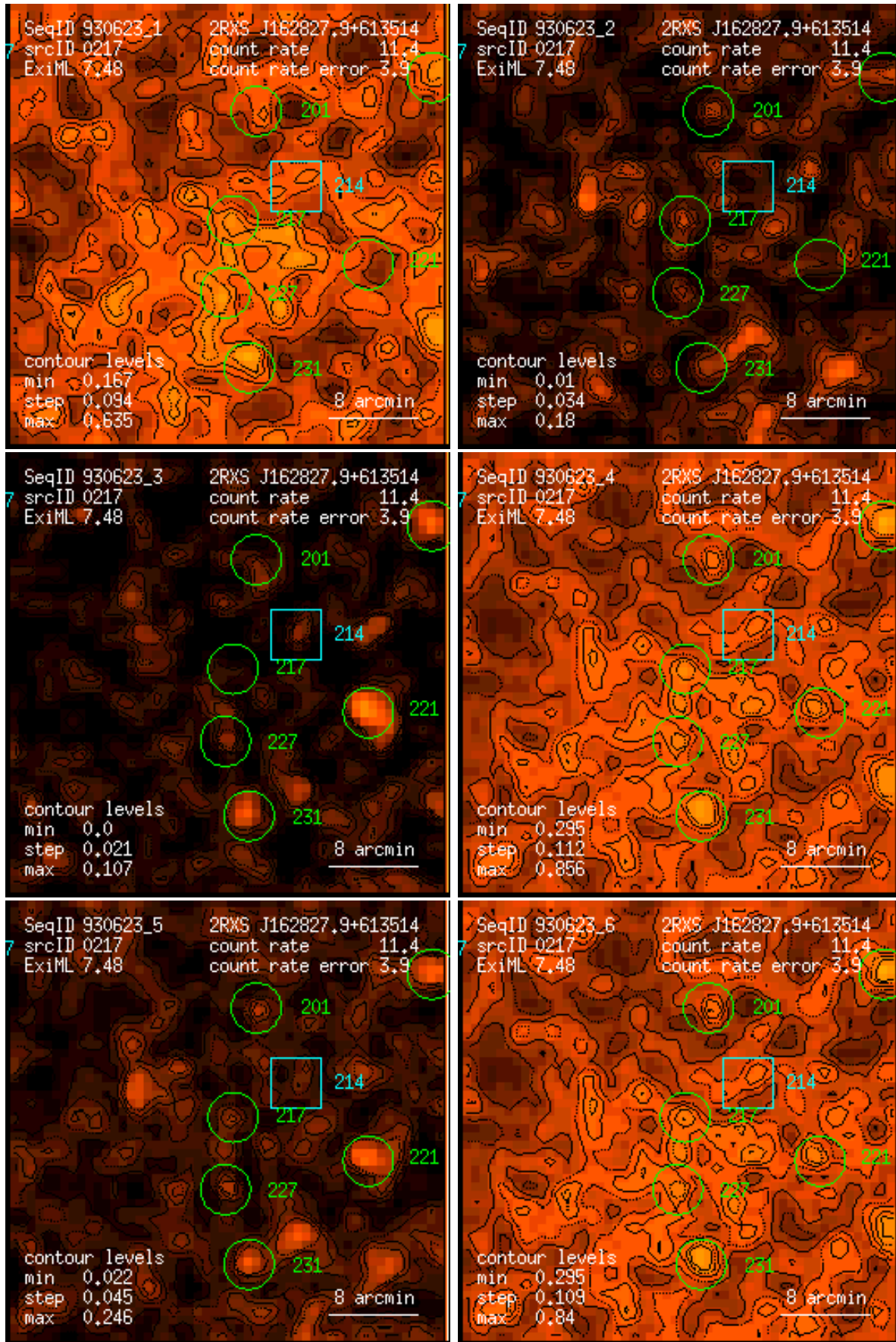
Figure 217: RASS 930623: detection 0217: band rate images, Gaussian filter: (1) PSPC channels 11 – 41, (2) 52 – 90, (3) 91 – 201, (4) 11 – 235, (5) 52 – 201, (6) 11 – 201. Broad band rates in counts/ks. Band rate contour levels in counts/ks/arcmin 2 .
