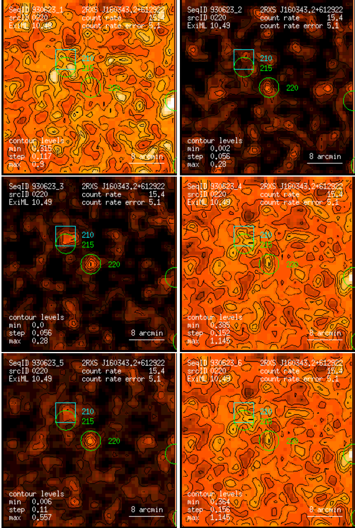
Figure 220: RASS 930623: detection 0220: band rate images, Gaussian filter: (1) PSPC channels 11 – 41, (2) 52 – 90, (3) 91 – 201, (4) 11 – 235, (5) 52 – 201, (6) 11 – 201. Broad band rates in counts/ks. Band rate contour levels in counts/ks/arcmin 2 .
