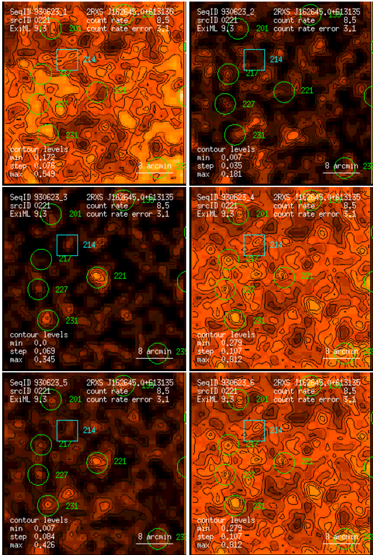
Figure 221: RASS 930623: detection 0221: band rate images, Gaussian filter: (1) PSPC channels 11 – 41, (2) 52 – 90, (3) 91 – 201, (4) 11 – 235, (5) 52 – 201, (6) 11 – 201. Broad band rates in counts/ks. Band rate contour levels in counts/ks/arcmin 2 .
