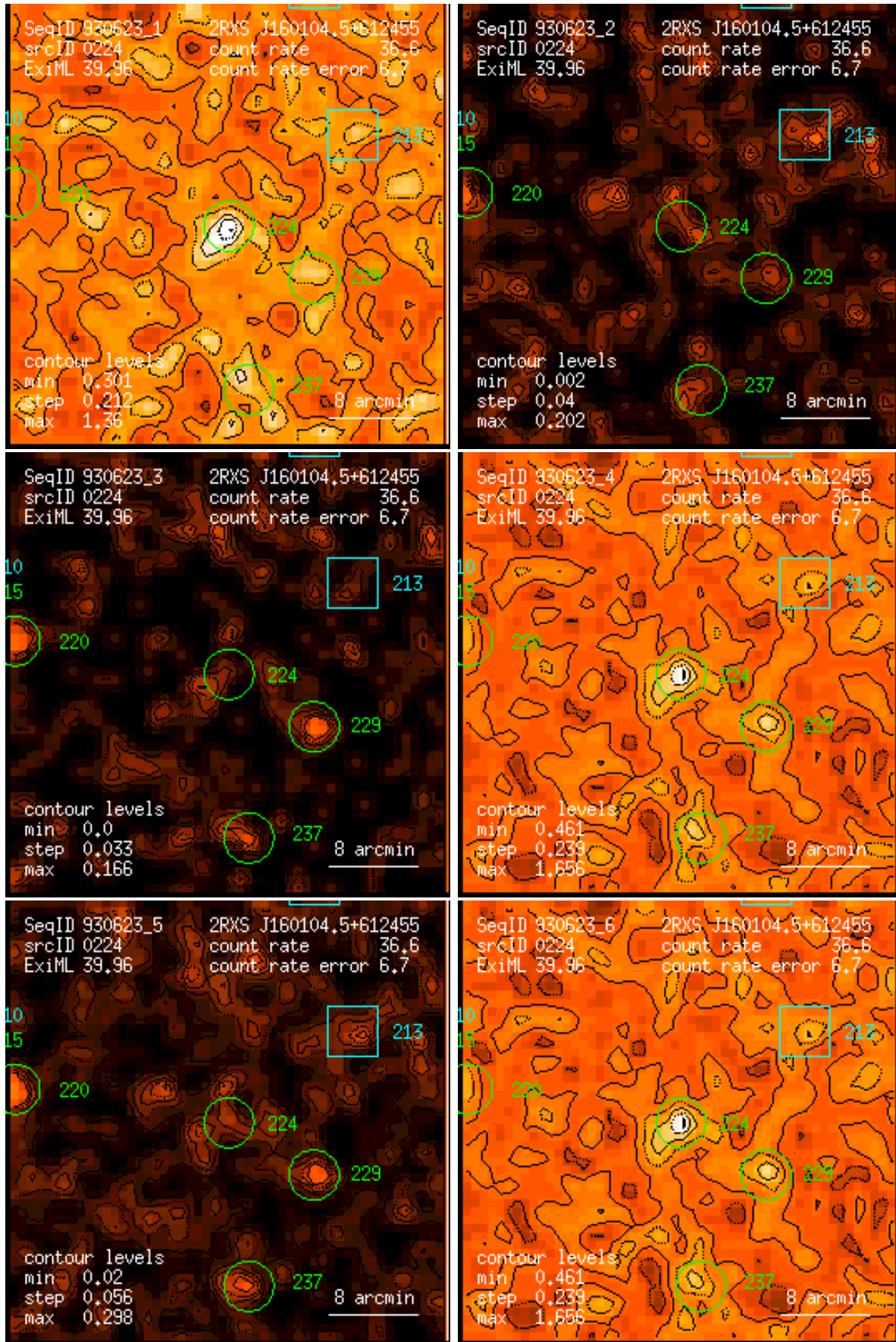
Figure 224: RASS 930623: detection 0224: band rate images, Gaussian filter: (1) PSPC channels 11 – 41, (2) 52 – 90, (3) 91 – 201, (4) 11 – 235, (5) 52 – 201, (6) 11 – 201. Broad band rates in counts/ks. Band rate contour levels in counts/ks/arcmin 2 .
