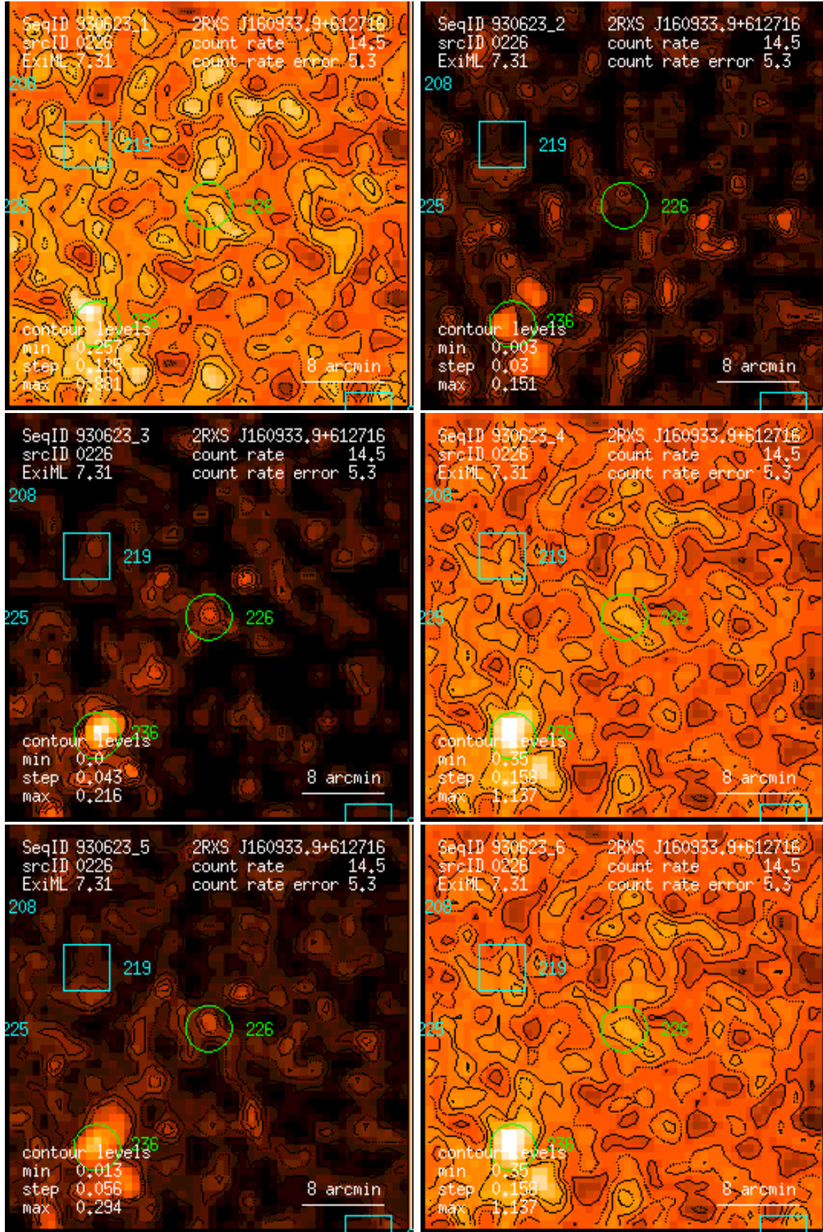
Figure 226: RASS 930623: detection 0226: band rate images, Gaussian filter: (1) PSPC channels 11 – 41, (2) 52 – 90, (3) 91 – 201, (4) 11 – 235, (5) 52 – 201, (6) 11 – 201. Broad band rates in counts/ks. Band rate contour levels in counts/ks/arcmin 2 .
