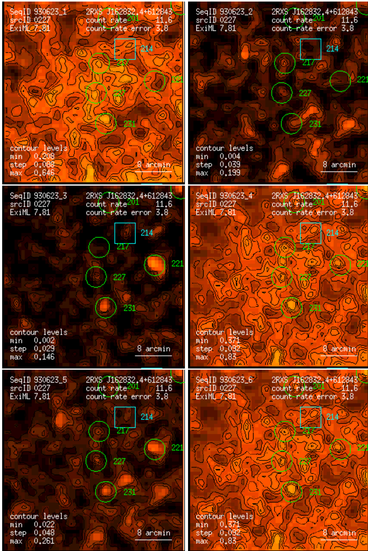
Figure 227: RASS 930623: detection 0227: band rate images, Gaussian filter: (1) PSPC channels 11 – 41, (2) 52 – 90, (3) 91 – 201, (4) 11 – 235, (5) 52 – 201, (6) 11 – 201. Broad band rates in counts/ks. Band rate contour levels in counts/ks/arcmin 2 .
