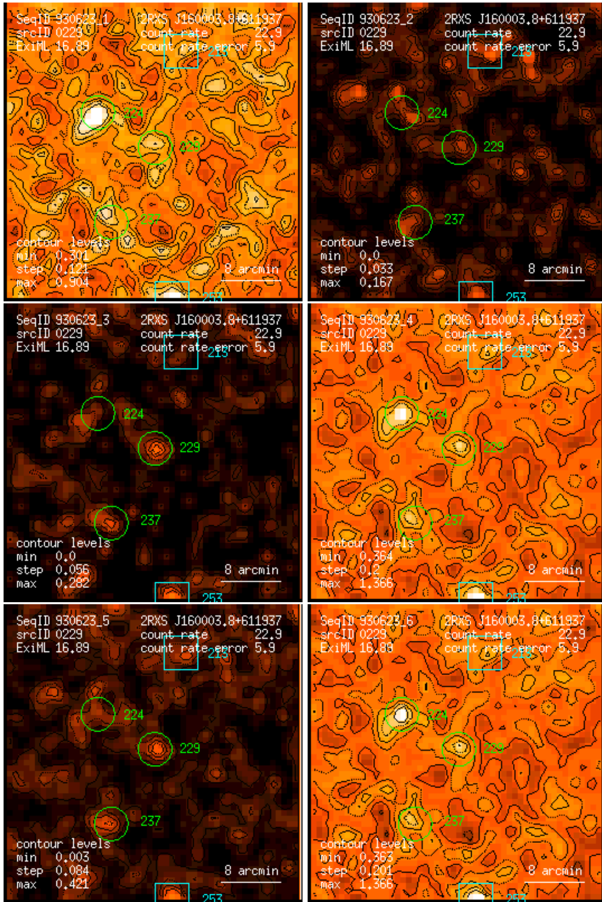
Figure 229: RASS 930623: detection 0229: band rate images, Gaussian filter: (1) PSPC channels 11 – 41, (2) 52 – 90, (3) 91 – 201, (4) 11 – 235, (5) 52 – 201, (6) 11 – 201. Broad band rates in counts/ks. Band rate contour levels in counts/ks/arcmin 2 .
