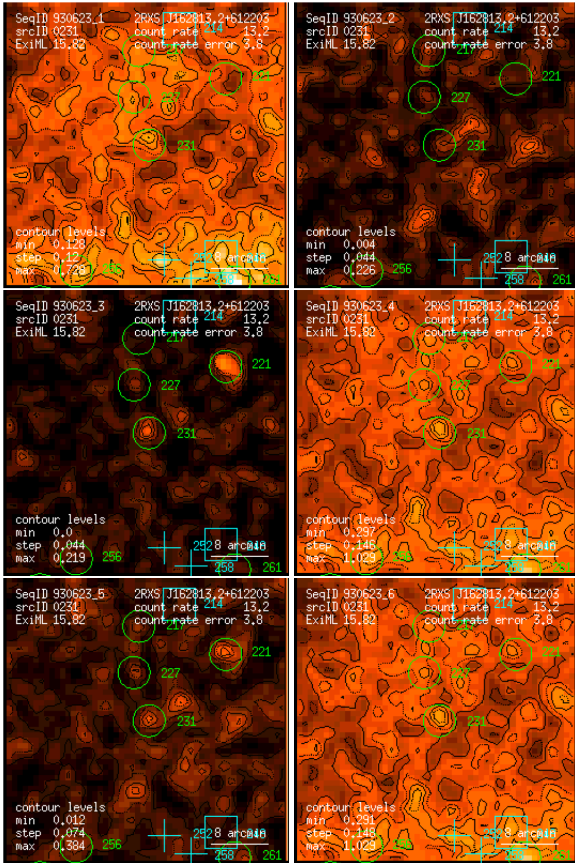
Figure 231: RASS 930623: detection 0231: band rate images, Gaussian filter: (1) PSPC channels 11 – 41, (2) 52 – 90, (3) 91 – 201, (4) 11 – 235, (5) 52 – 201, (6) 11 – 201. Broad band rates in counts/ks. Band rate contour levels in counts/ks/arcmin 2 .
