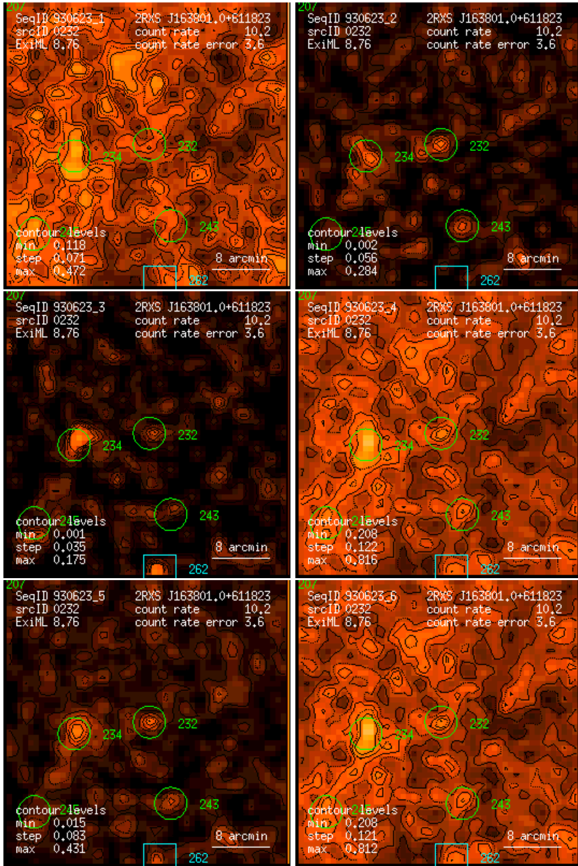
Figure 232: RASS 930623: detection 0232: band rate images, Gaussian filter: (1) PSPC channels 11 – 41, (2) 52 – 90, (3) 91 – 201, (4) 11 – 235, (5) 52 – 201, (6) 11 – 201. Broad band rates in counts/ks. Band rate contour levels in counts/ks/arcmin 2 .
