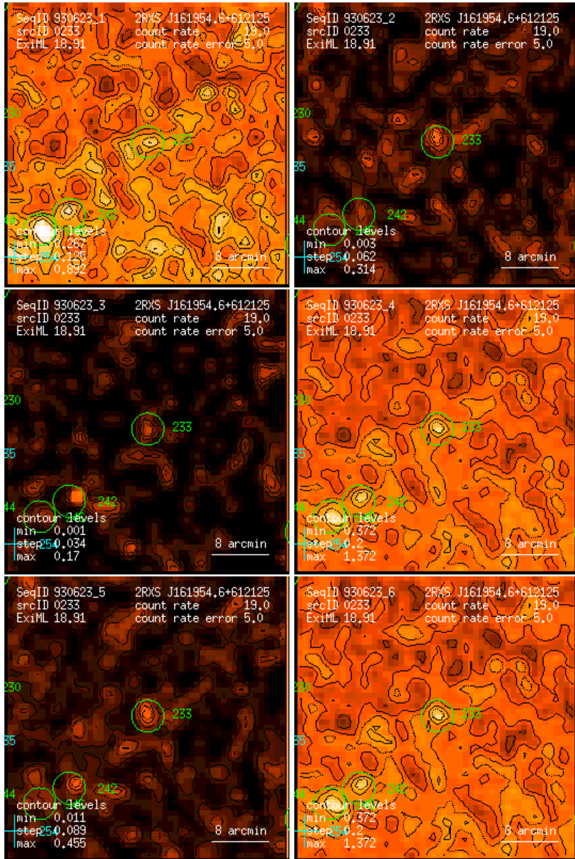
Figure 233: RASS 930623: detection 0233: band rate images, Gaussian filter: (1) PSPC channels 11 – 41, (2) 52 – 90, (3) 91 – 201, (4) 11 – 235, (5) 52 – 201, (6) 11 – 201. Broad band rates in counts/ks. Band rate contour levels in counts/ks/arcmin 2 .
