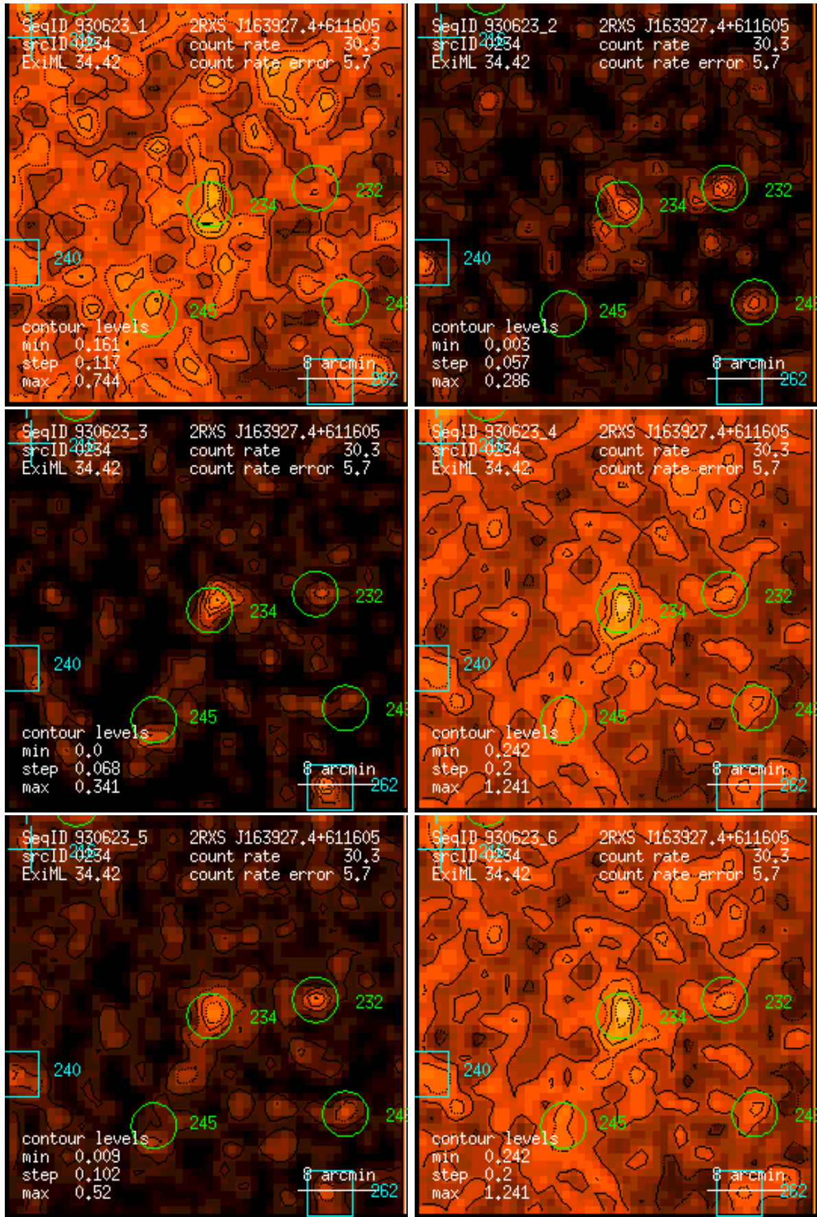
Figure 234: RASS 930623: detection 0234: band rate images, Gaussian filter: (1) PSPC channels 11 – 41, (2) 52 – 90, (3) 91 – 201, (4) 11 – 235, (5) 52 – 201, (6) 11 – 201. Broad band rates in counts/ks. Band rate contour levels in counts/ks/arcmin 2 .
