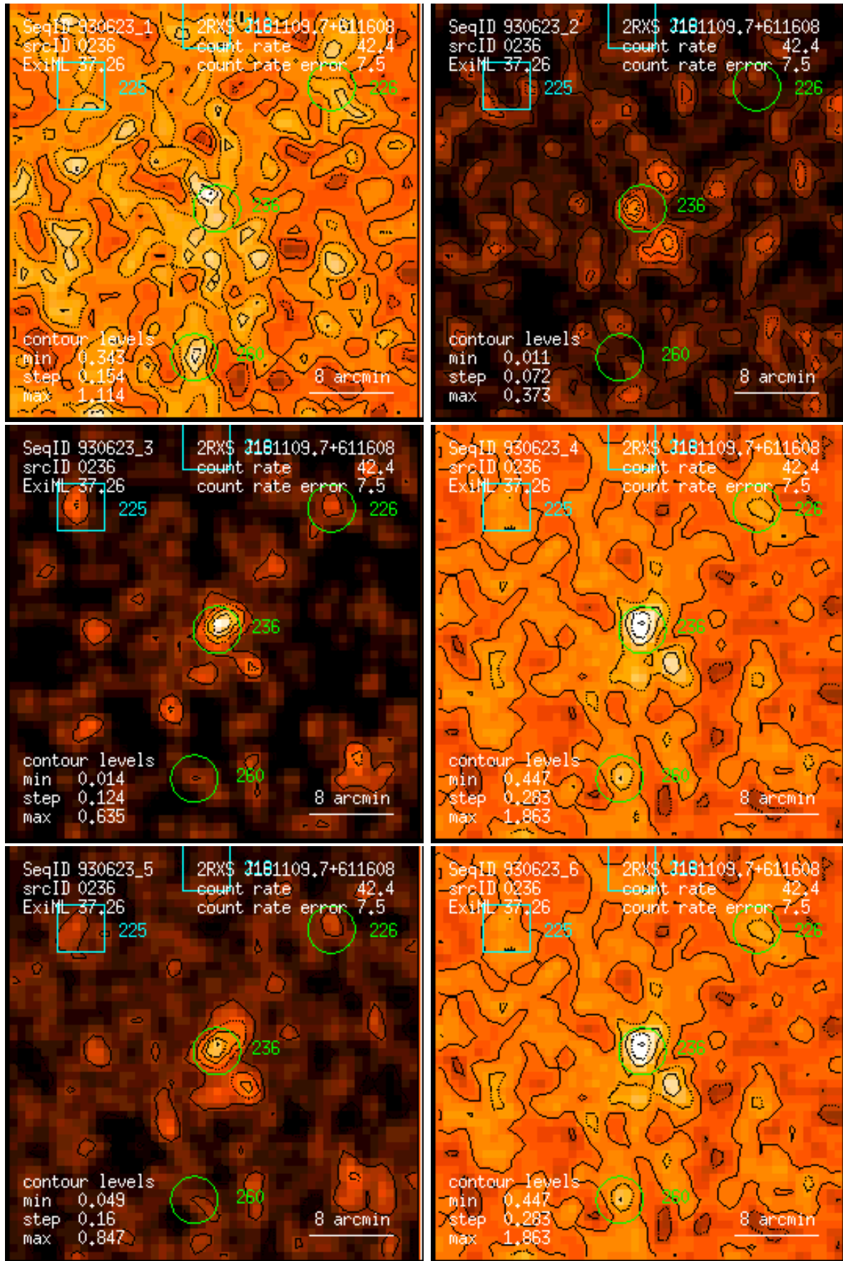
Figure 236: RASS 930623: detection 0236: band rate images, Gaussian filter: (1) PSPC channels 11 – 41, (2) 52 – 90, (3) 91 – 201, (4) 11 – 235, (5) 52 – 201, (6) 11 – 201. Broad band rates in counts/ks. Band rate contour levels in counts/ks/arcmin 2 .
