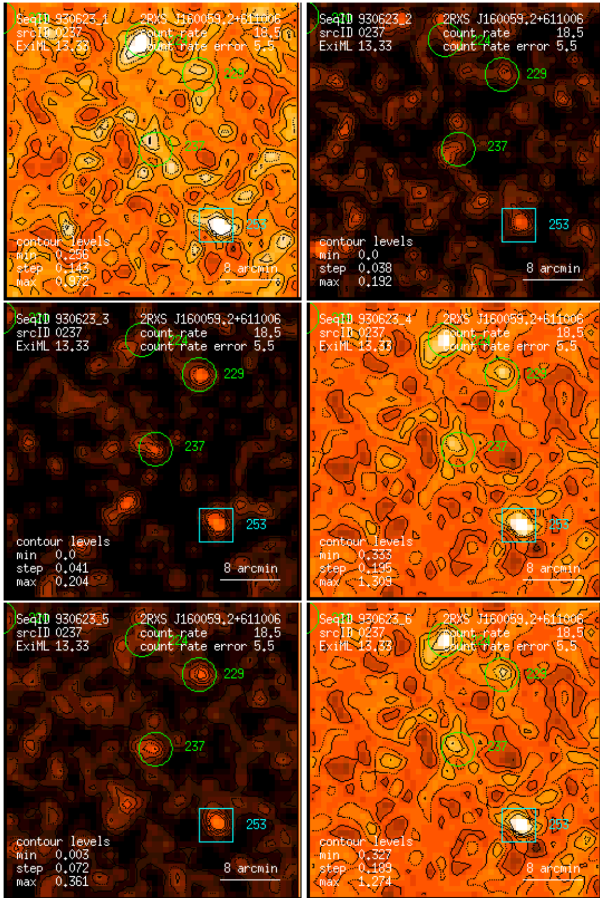
Figure 237: RASS 930623: detection 0237: band rate images, Gaussian filter: (1) PSPC channels 11 – 41, (2) 52 – 90, (3) 91 – 201, (4) 11 – 235, (5) 52 – 201, (6) 11 – 201. Broad band rates in counts/ks. Band rate contour levels in counts/ks/arcmin 2 .
