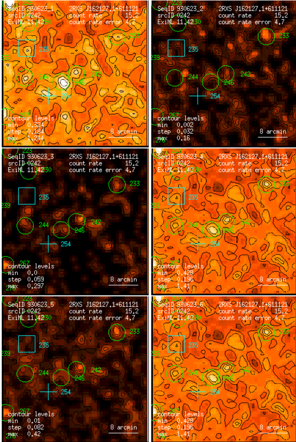
Figure 242: RASS 930623: detection 0242: band rate images, Gaussian filter: (1) PSPC channels 11 – 41, (2) 52 – 90, (3) 91 – 201, (4) 11 – 235, (5) 52 – 201, (6) 11 – 201. Broad band rates in counts/ks. Band rate contour levels in counts/ks/arcmin 2 .
