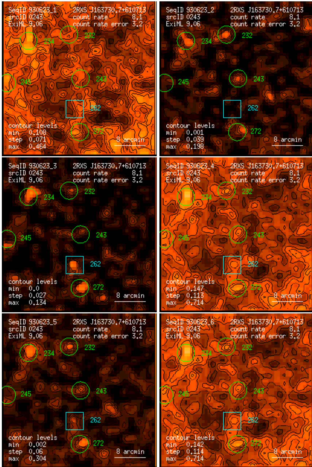
Figure 243: RASS 930623: detection 0243: band rate images, Gaussian filter: (1) PSPC channels 11 – 41, (2) 52 – 90, (3) 91 – 201, (4) 11 – 235, (5) 52 – 201, (6) 11 – 201. Broad band rates in counts/ks. Band rate contour levels in counts/ks/arcmin 2 .
