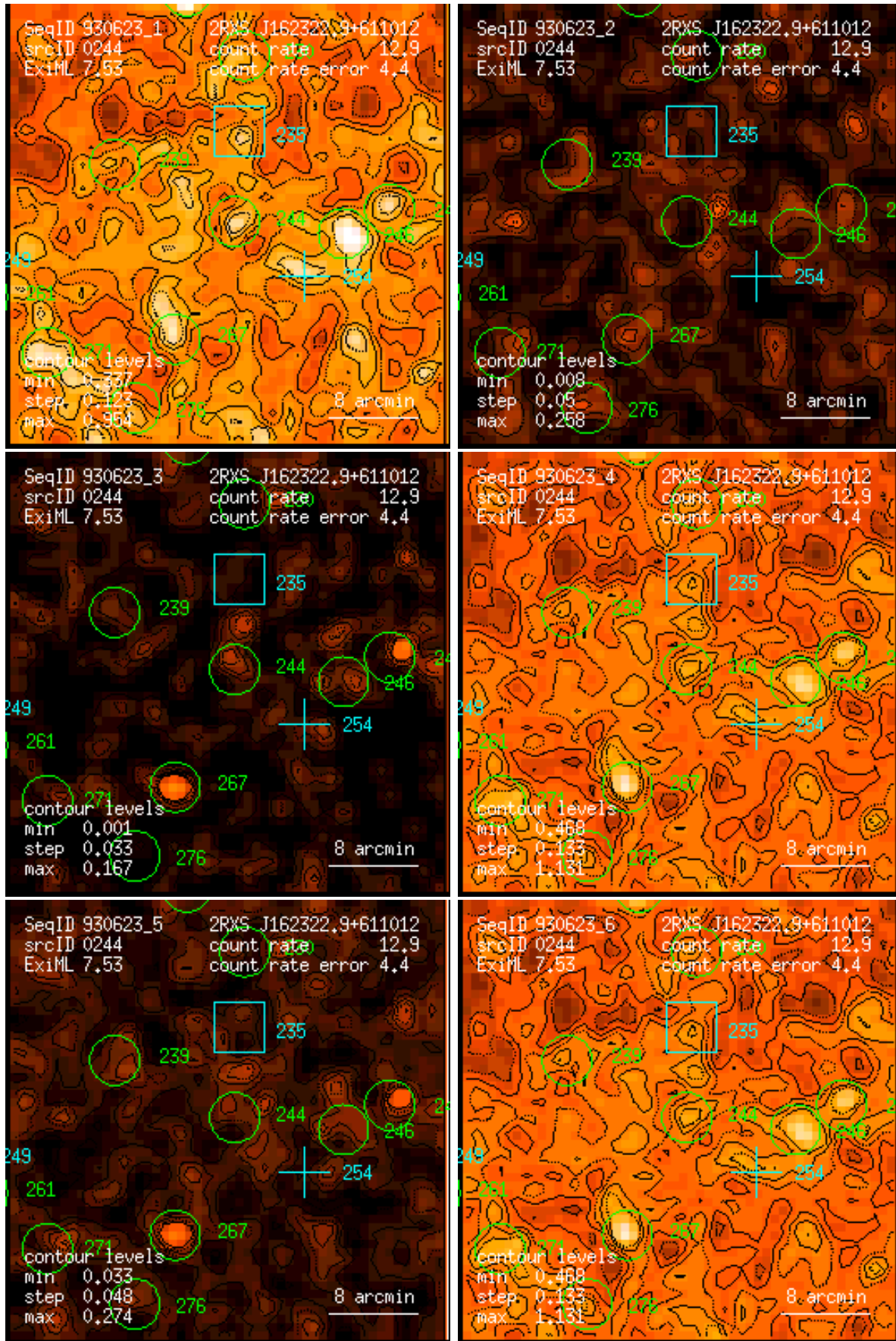
Figure 244: RASS 930623: detection 0244: band rate images, Gaussian filter: (1) PSPC channels 11 – 41, (2) 52 – 90, (3) 91 – 201, (4) 11 – 235, (5) 52 – 201, (6) 11 – 201. Broad band rates in counts/ks. Band rate contour levels in counts/ks/arcmin 2 .
