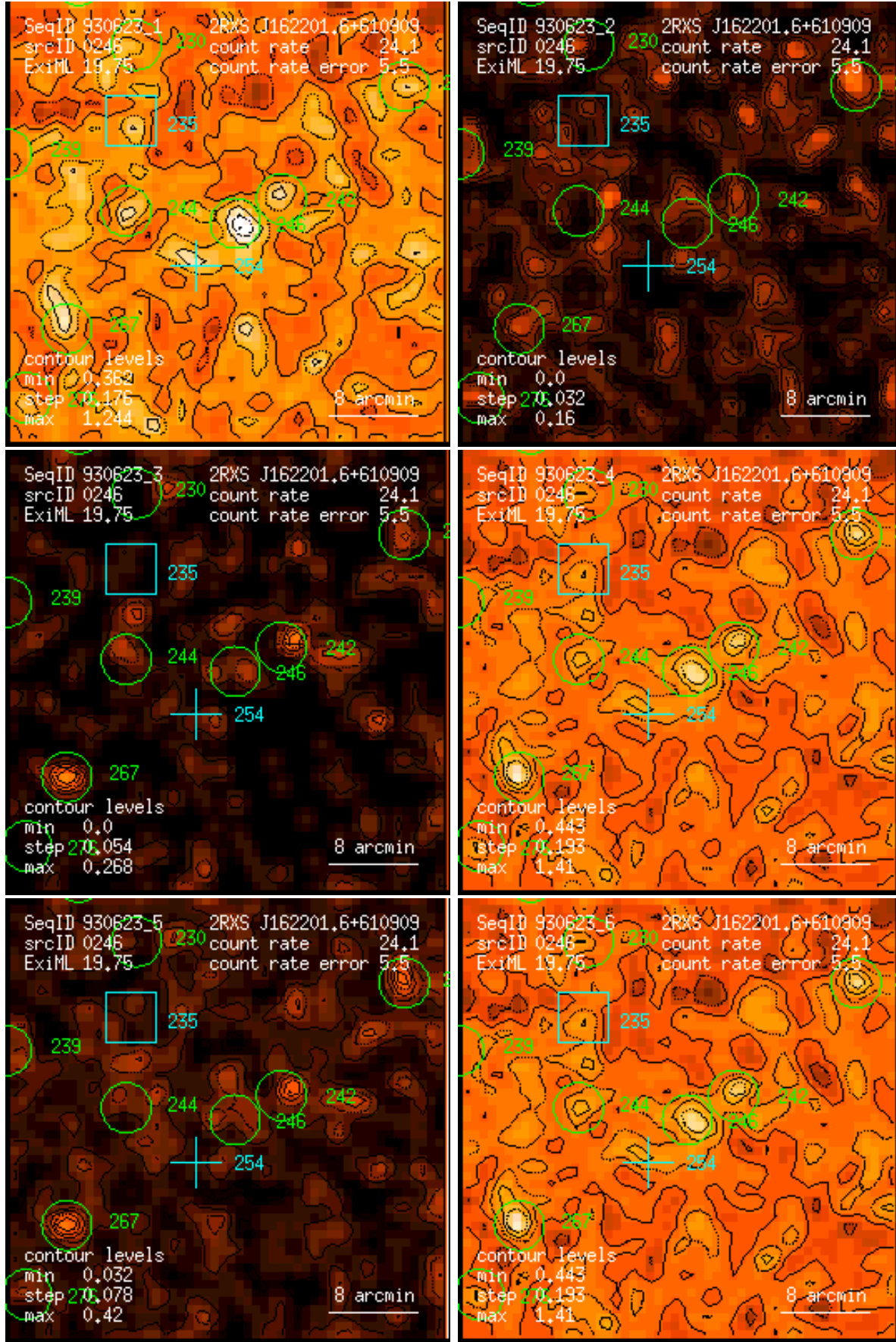
Figure 246: RASS 930623: detection 0246: band rate images, Gaussian filter: (1) PSPC channels 11 – 41, (2) 52 – 90, (3) 91 – 201, (4) 11 – 235, (5) 52 – 201, (6) 11 – 201. Broad band rates in counts/ks. Band rate contour levels in counts/ks/arcmin 2 .
