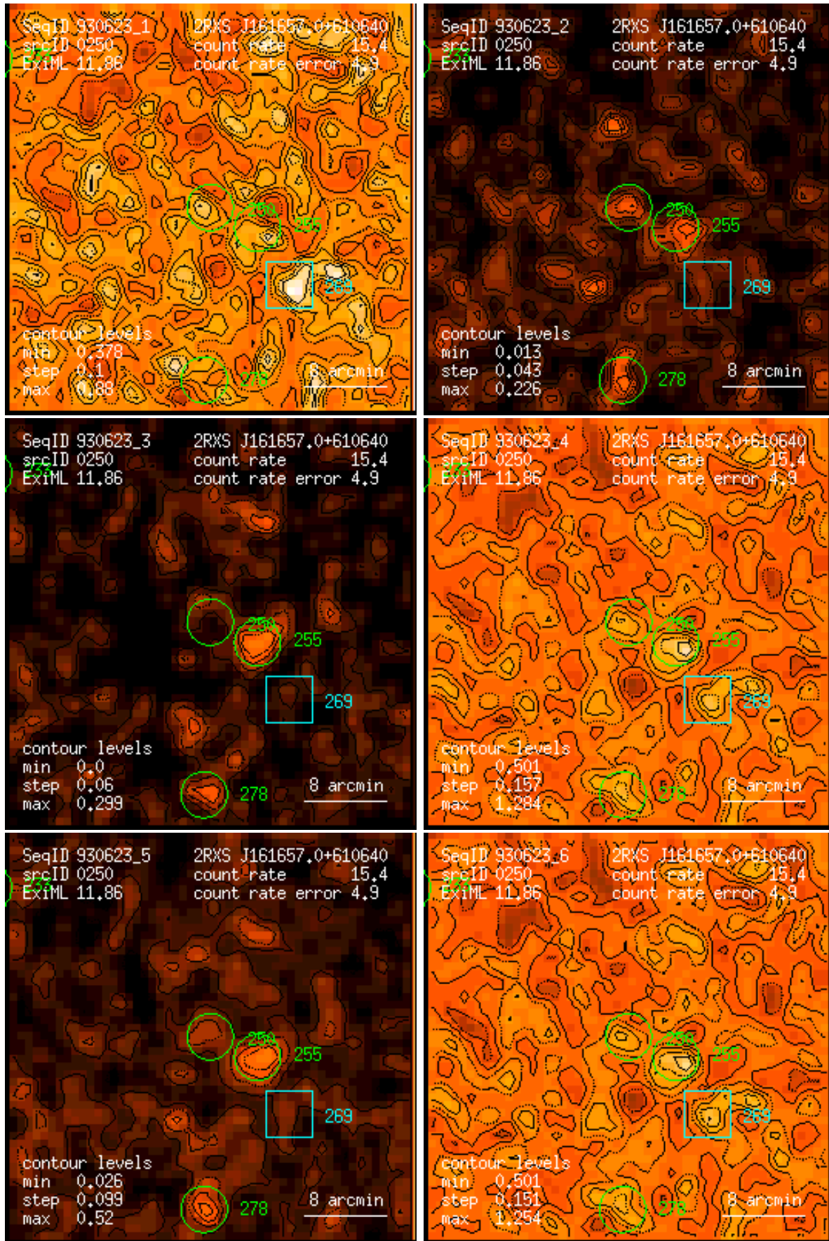
Figure 250: RASS 930623: detection 0250: band rate images, Gaussian filter: (1) PSPC channels 11 – 41, (2) 52 – 90, (3) 91 – 201, (4) 11 – 235, (5) 52 – 201, (6) 11 – 201. Broad band rates in counts/ks. Band rate contour levels in counts/ks/arcmin 2 .
