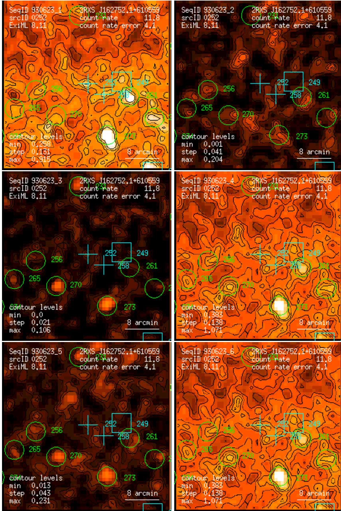
Figure 252: RASS 930623: detection 0252: band rate images, Gaussian filter: (1) PSPC channels 11 – 41, (2) 52 – 90, (3) 91 – 201, (4) 11 – 235, (5) 52 – 201, (6) 11 – 201. Broad band rates in counts/ks. Band rate contour levels in counts/ks/arcmin 2 .
