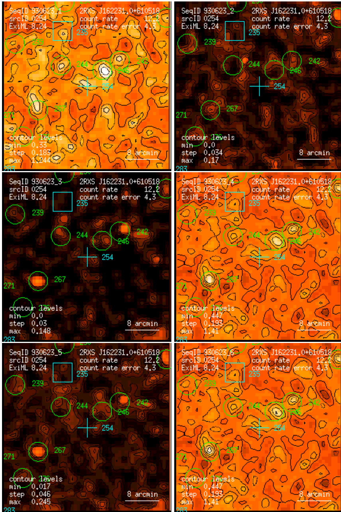
Figure 254: RASS 930623: detection 0254: band rate images, Gaussian filter: (1) PSPC channels 11 – 41, (2) 52 – 90, (3) 91 – 201, (4) 11 – 235, (5) 52 – 201, (6) 11 – 201. Broad band rates in counts/ks. Band rate contour levels in counts/ks/arcmin 2 .
