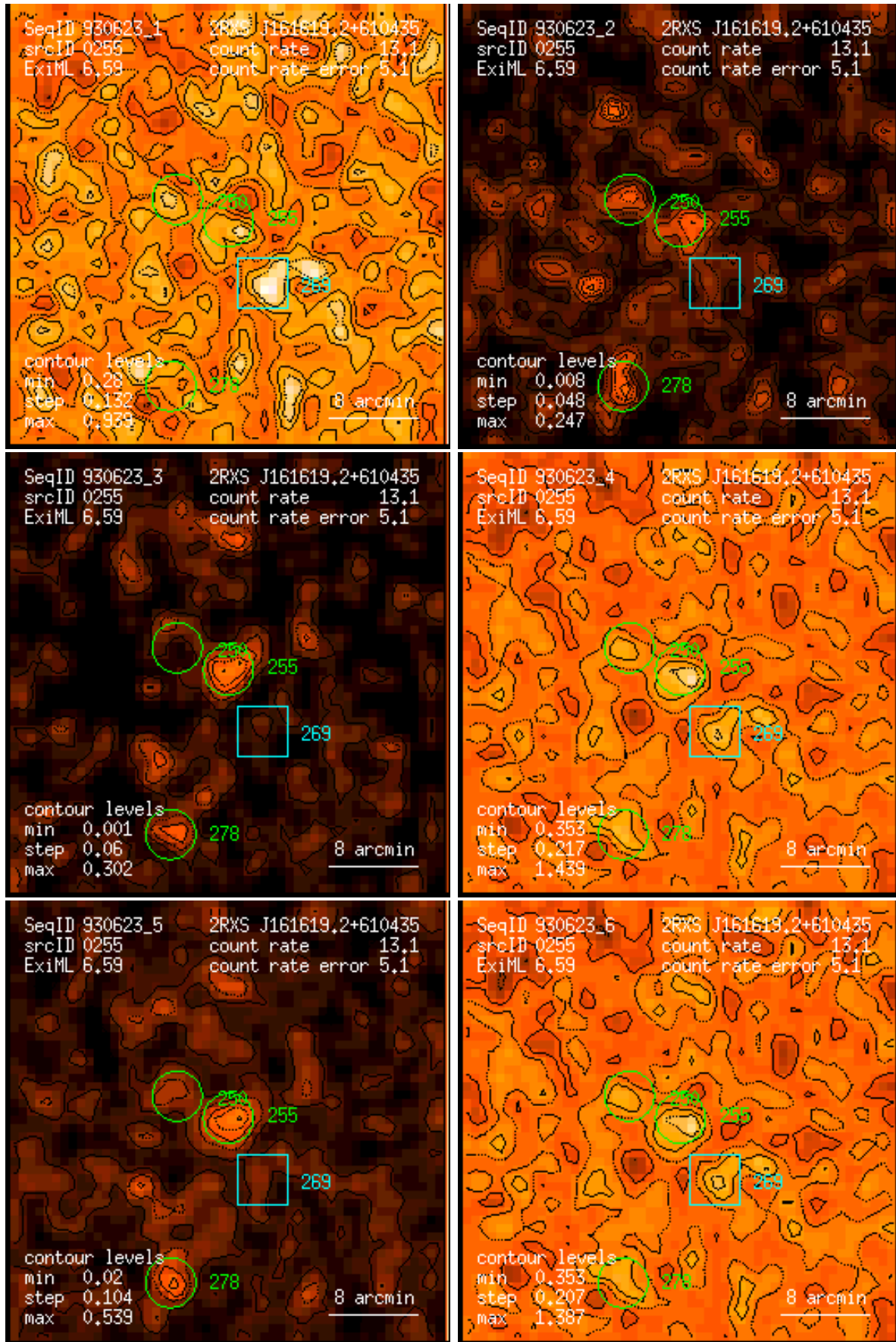
Figure 255: RASS 930623: detection 0255: band rate images, Gaussian filter: (1) PSPC channels 11 – 41, (2) 52 – 90, (3) 91 – 201, (4) 11 – 235, (5) 52 – 201, (6) 11 – 201. Broad band rates in counts/ks. Band rate contour levels in counts/ks/arcmin 2 .
