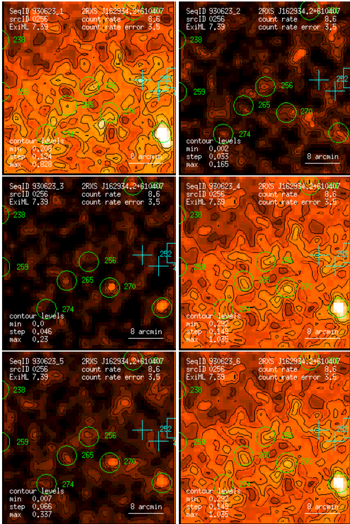
Figure 256: RASS 930623: detection 0256: band rate images, Gaussian filter: (1) PSPC channels 11 – 41, (2) 52 – 90, (3) 91 – 201, (4) 11 – 235, (5) 52 – 201, (6) 11 – 201. Broad band rates in counts/ks. Band rate contour levels in counts/ks/arcmin 2 .
