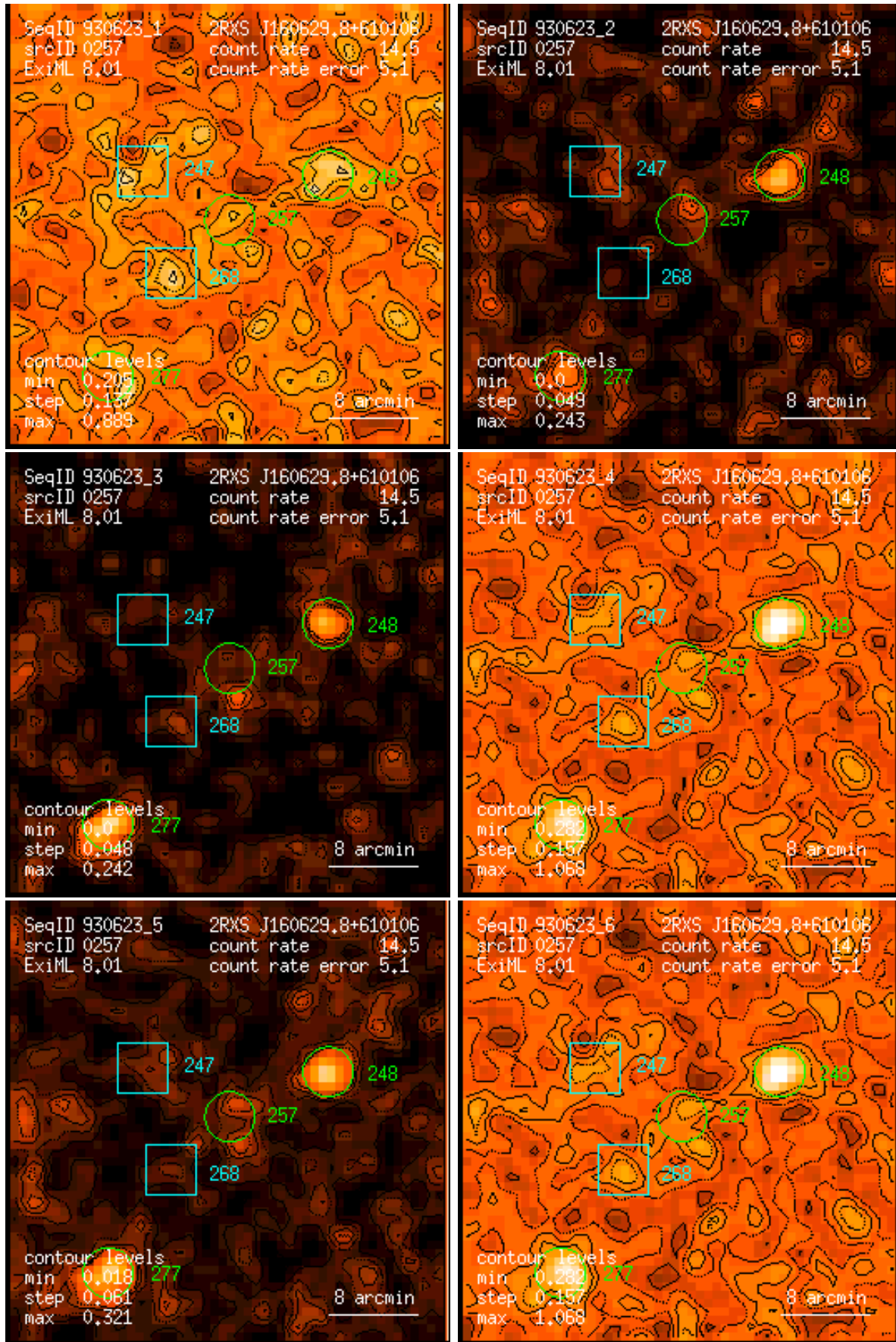
Figure 257: RASS 930623: detection 0257: band rate images, Gaussian filter: (1) PSPC channels 11 – 41, (2) 52 – 90, (3) 91 – 201, (4) 11 – 235, (5) 52 – 201, (6) 11 – 201. Broad band rates in counts/ks. Band rate contour levels in counts/ks/arcmin 2 .
