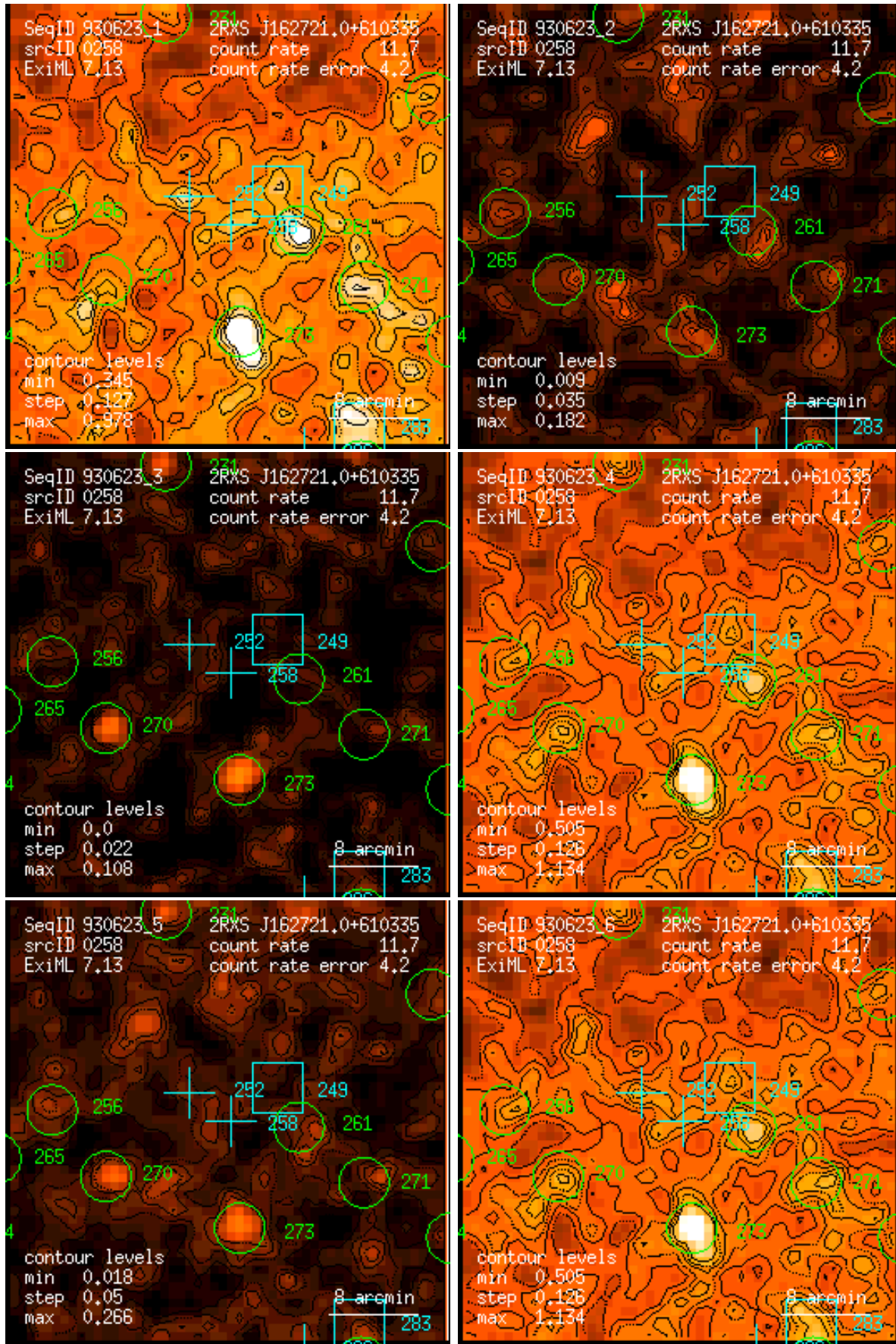
Figure 258: RASS 930623: detection 0258: band rate images, Gaussian filter: (1) PSPC channels 11 – 41, (2) 52 – 90, (3) 91 – 201, (4) 11 – 235, (5) 52 – 201, (6) 11 – 201. Broad band rates in counts/ks. Band rate contour levels in counts/ks/arcmin 2 .
