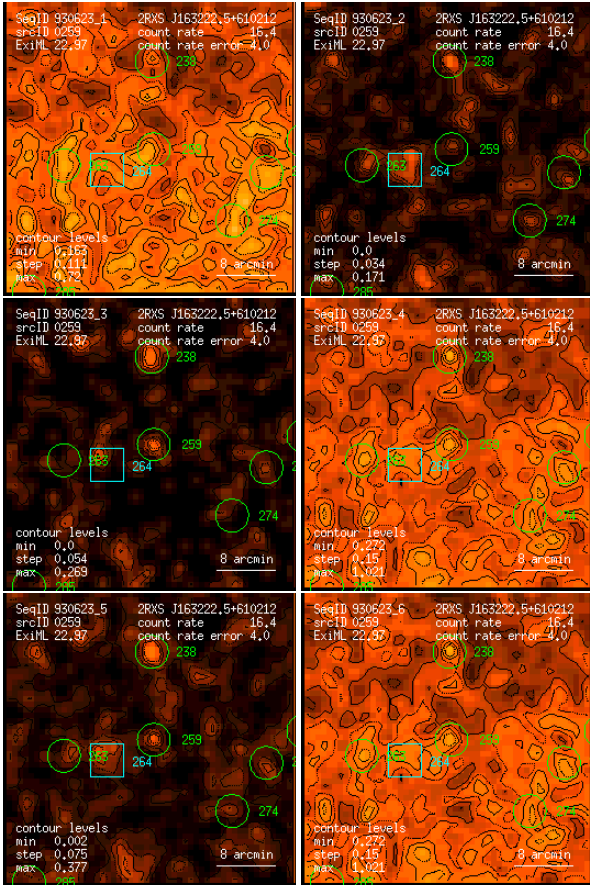
Figure 259: RASS 930623: detection 0259: band rate images, Gaussian filter: (1) PSPC channels 11 – 41, (2) 52 – 90, (3) 91 – 201, (4) 11 – 235, (5) 52 – 201, (6) 11 – 201. Broad band rates in counts/ks. Band rate contour levels in counts/ks/arcmin 2 .
