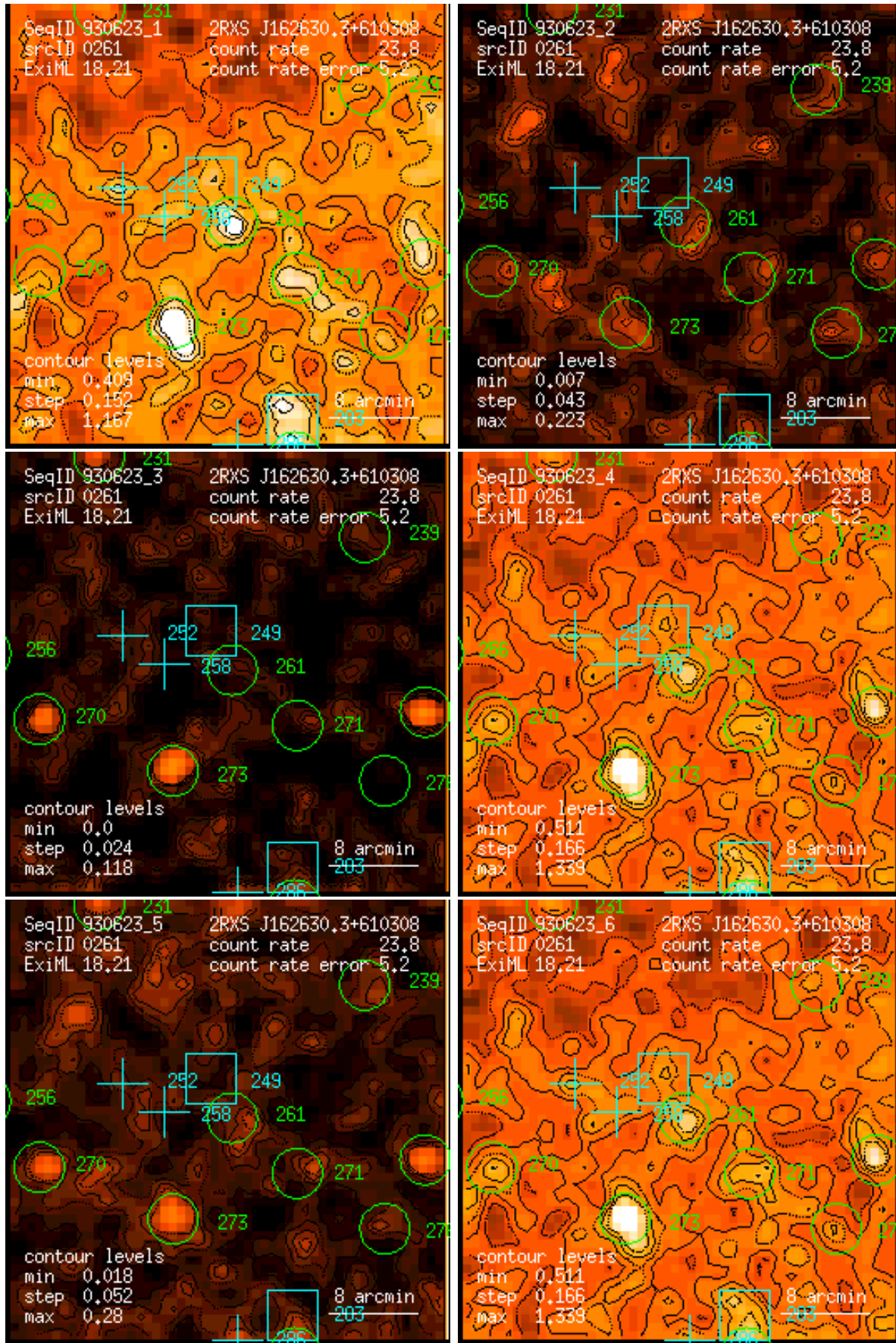
Figure 261: RASS 930623: detection 0261: band rate images, Gaussian filter: (1) PSPC channels 11 – 41, (2) 52 – 90, (3) 91 – 201, (4) 11 – 235, (5) 52 – 201, (6) 11 – 201. Broad band rates in counts/ks. Band rate contour levels in counts/ks/arcmin 2 .
