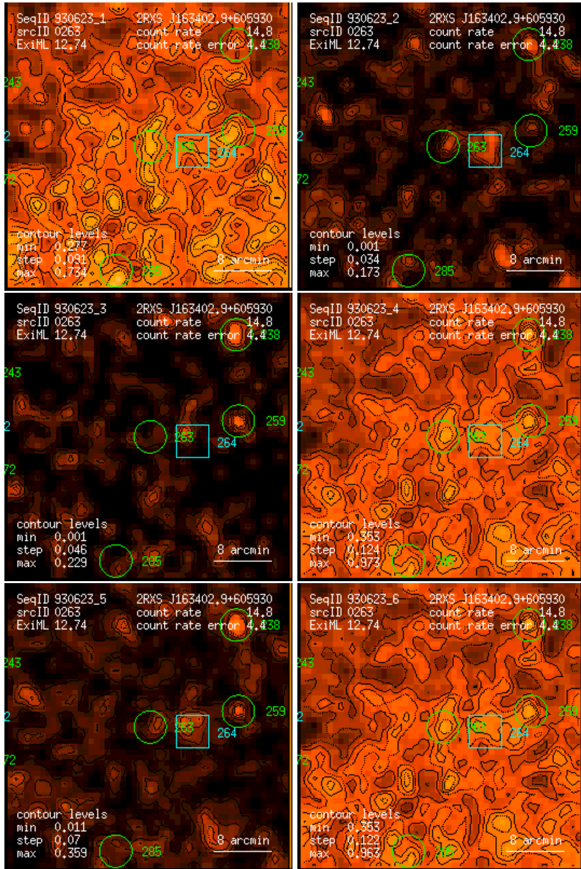
Figure 263: RASS 930623: detection 0263: band rate images, Gaussian filter: (1) PSPC channels 11 – 41, (2) 52 – 90, (3) 91 – 201, (4) 11 – 235, (5) 52 – 201, (6) 11 – 201. Broad band rates in counts/ks. Band rate contour levels in counts/ks/arcmin 2 .
