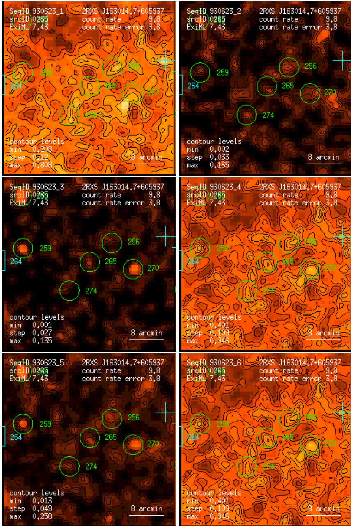
Figure 265: RASS 930623: detection 0265: band rate images, Gaussian filter: (1) PSPC channels 11 – 41, (2) 52 – 90, (3) 91 – 201, (4) 11 – 235, (5) 52 – 201, (6) 11 – 201. Broad band rates in counts/ks. Band rate contour levels in counts/ks/arcmin 2 .
