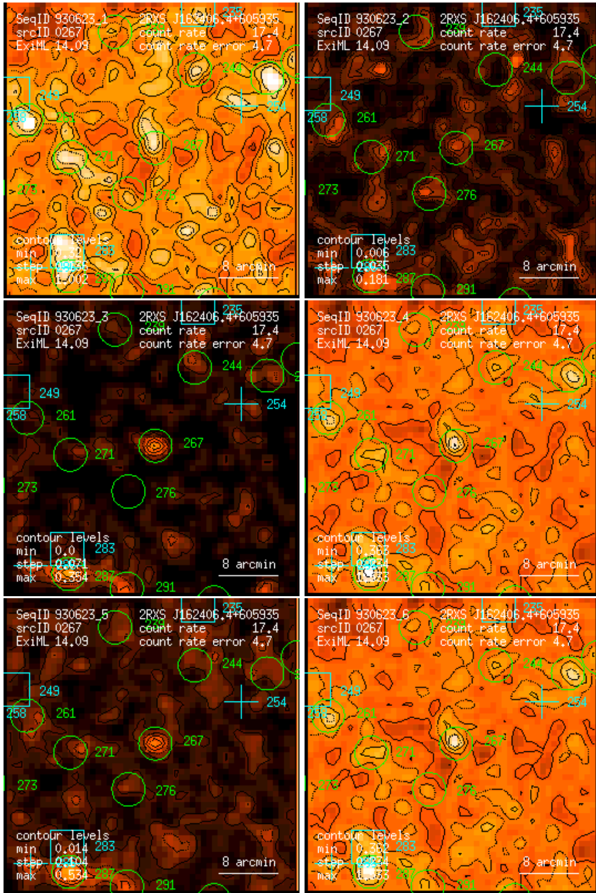
Figure 267: RASS 930623: detection 0267: band rate images, Gaussian filter: (1) PSPC channels 11 – 41, (2) 52 – 90, (3) 91 – 201, (4) 11 – 235, (5) 52 – 201, (6) 11 – 201. Broad band rates in counts/ks. Band rate contour levels in counts/ks/arcmin 2 .
