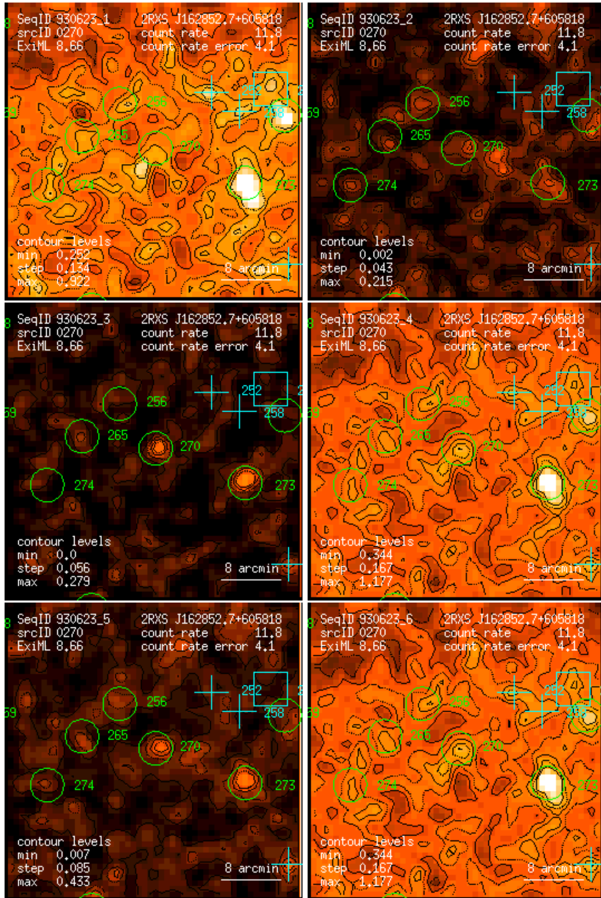
Figure 270: RASS 930623: detection 0270: band rate images, Gaussian filter: (1) PSPC channels 11 – 41, (2) 52 – 90, (3) 91 – 201, (4) 11 – 235, (5) 52 – 201, (6) 11 – 201. Broad band rates in counts/ks. Band rate contour levels in counts/ks/arcmin 2 .
