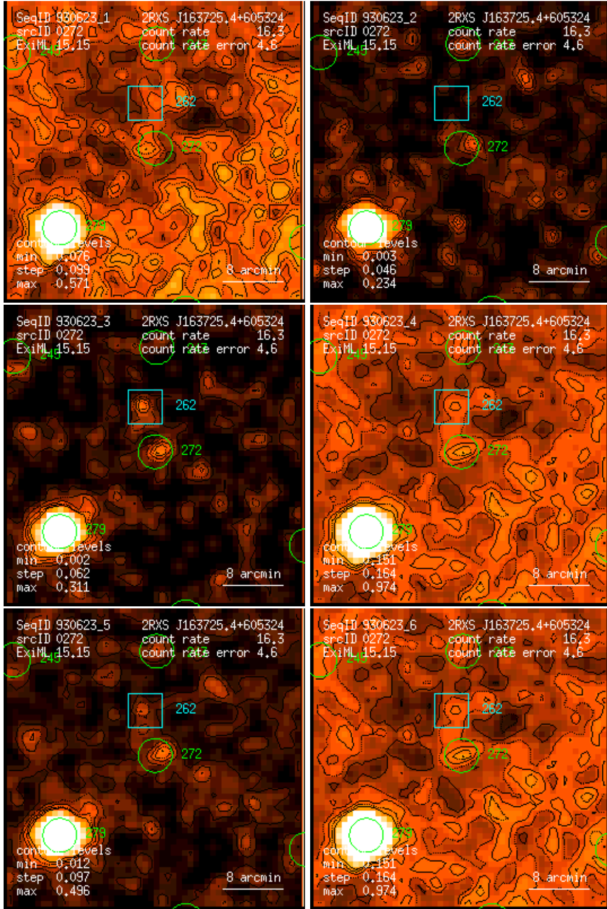
Figure 272: RASS 930623: detection 0272: band rate images, Gaussian filter: (1) PSPC channels 11 – 41, (2) 52 – 90, (3) 91 – 201, (4) 11 – 235, (5) 52 – 201, (6) 11 – 201. Broad band rates in counts/ks. Band rate contour levels in counts/ks/arcmin 2 .
