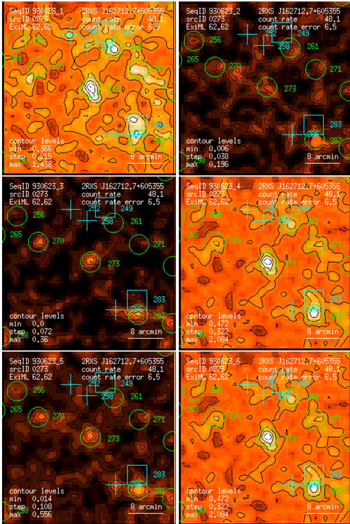
Figure 273: RASS 930623: detection 0273: band rate images, Gaussian filter: (1) PSPC channels 11 – 41, (2) 52 – 90, (3) 91 – 201, (4) 11 – 235, (5) 52 – 201, (6) 11 – 201. Broad band rates in counts/ks. Band rate contour levels in counts/ks/arcmin 2 .
