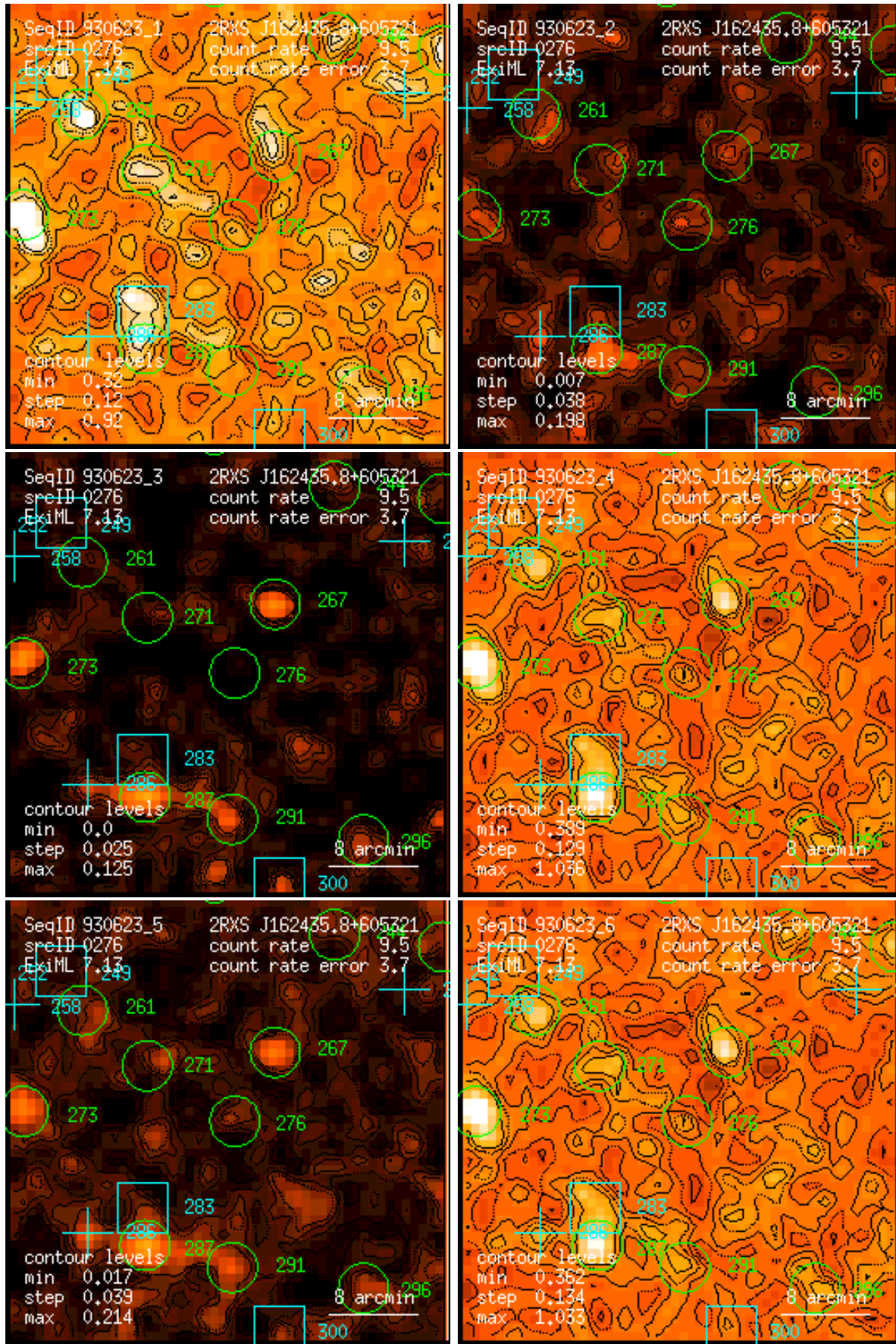
Figure 276: RASS 930623: detection 0276: band rate images, Gaussian filter: (1) PSPC channels 11 – 41, (2) 52 – 90, (3) 91 – 201, (4) 11 – 235, (5) 52 – 201, (6) 11 – 201. Broad band rates in counts/ks. Band rate contour levels in counts/ks/arcmin 2 .
