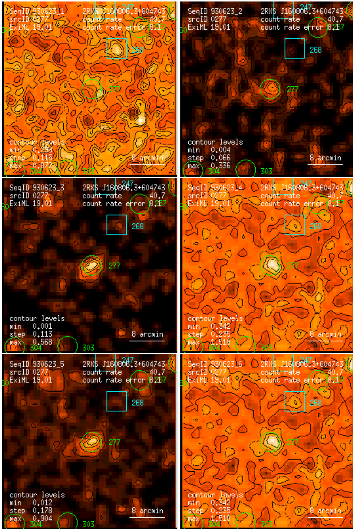
Figure 277: RASS 930623: detection 0277: band rate images, Gaussian filter: (1) PSPPC channels 11 – 41, (2) 52 – 90, (3) 91 – 201, (4) 11 – 235, (5) 52 – 201, (6) 11 – 201. Broad band rates in counts/ks. Band rate contour levels in counts/ks/arcmin 2 .
