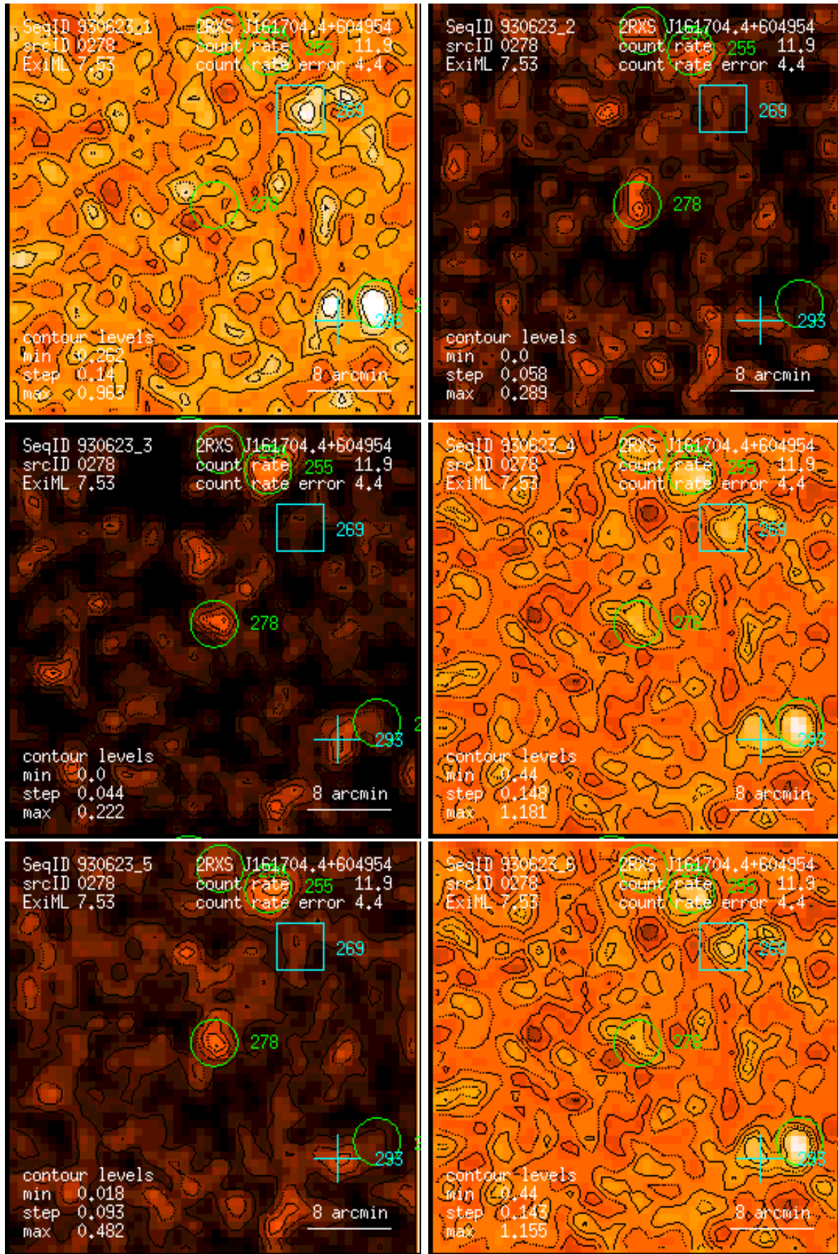
Figure 278: RASS 930623: detection 0278: band rate images, Gaussian filter: (1) PSPC channels 11 – 41, (2) 52 – 90, (3) 91 – 201, (4) 11 – 235, (5) 52 – 201, (6) 11 – 201. Broad band rates in counts/ks. Band rate contour levels in counts/ks/arcmin 2 .
