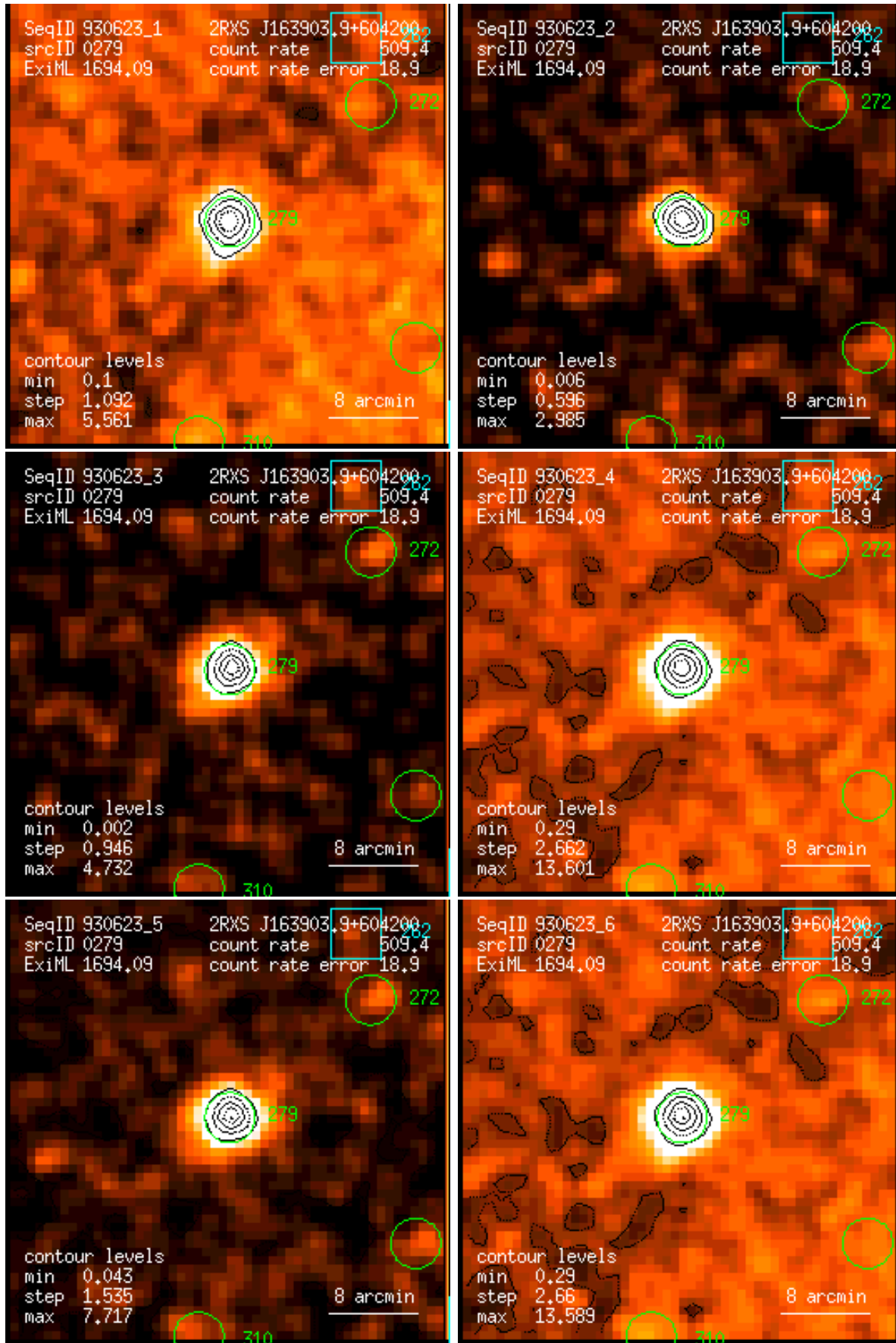
Figure 279: RASS 930623: detection 0279: band rate images, Gaussian filter: (1) PSPC channels 11 – 41, (2) 52 – 90, (3) 91 – 201, (4) 11 – 235, (5) 52 – 201, (6) 11 – 201. Broad band rates in counts/ks. Band rate contour levels in counts/ks/arcmin 2 .
