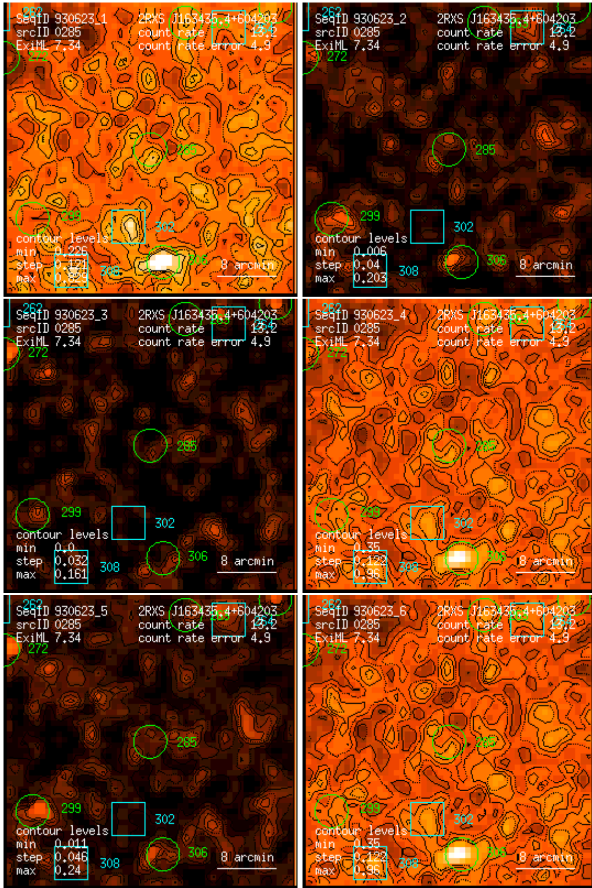
Figure 285: RASS 930623: detection 0285: band rate images, Gaussian filter: (1) PSPC channels 11 – 41, (2) 52 – 90, (3) 91 – 201, (4) 11 – 235, (5) 52 – 201, (6) 11 – 201. Broad band rates in counts/ks. Band rate contour levels in counts/ks/arcmin 2 .
