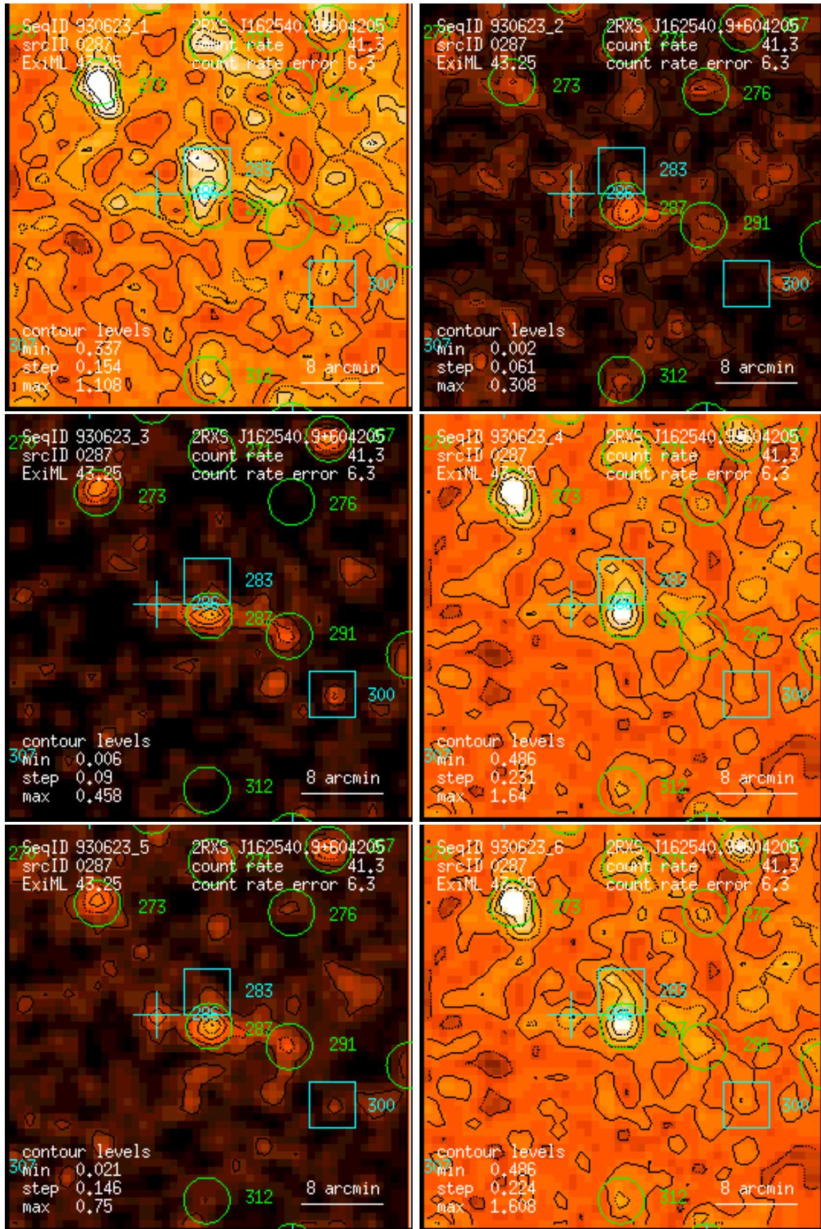
Figure 287: RASS 930623: detection 0287: band rate images, Gaussian filter: (1) PSPC channels 11 – 41, (2) 52 – 90, (3) 91 – 201, (4) 11 – 235, (5) 52 – 201, (6) 11 – 201. Broad band rates in counts/ks. Band rate contour levels in counts/ks/arcmin 2 .
