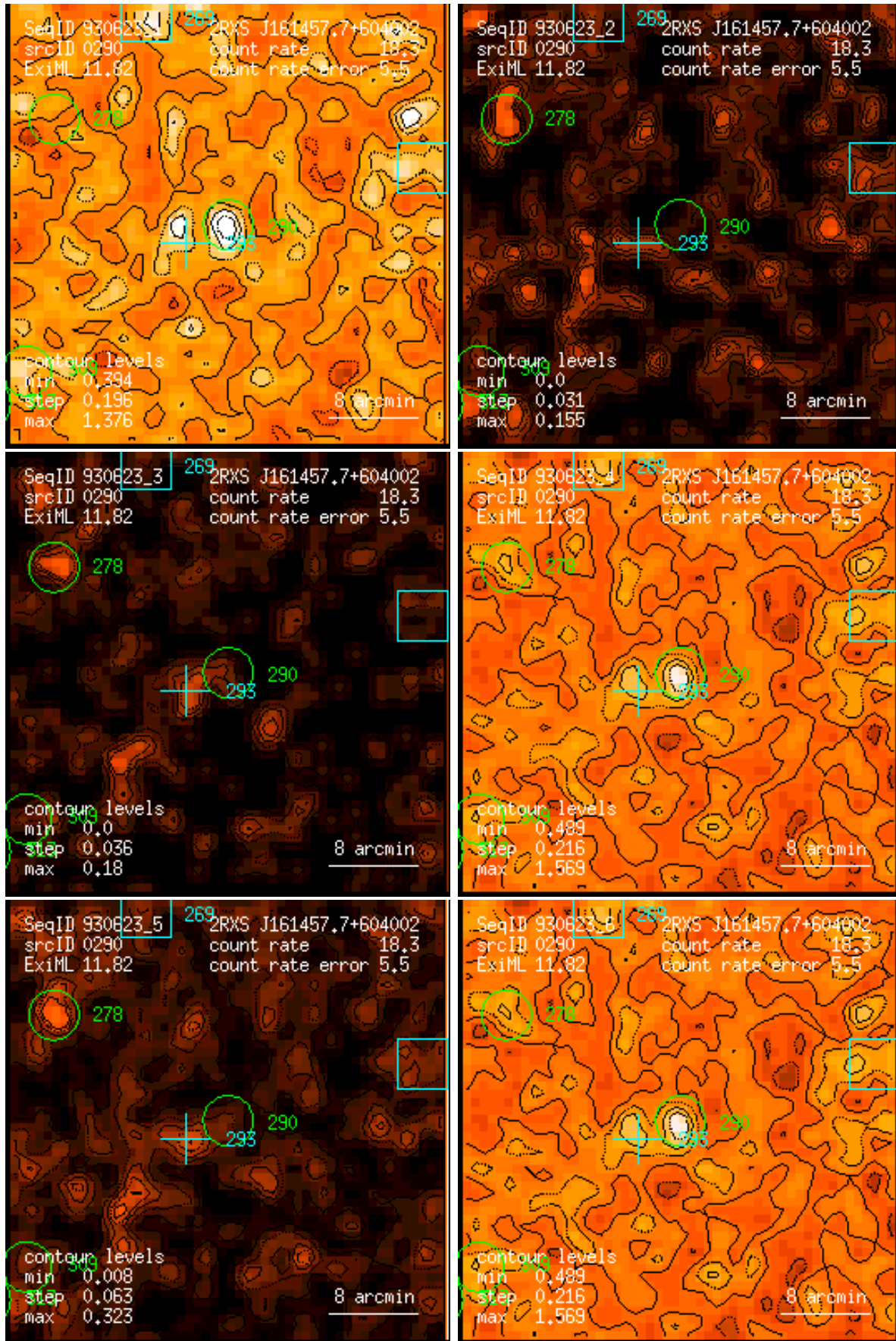
Figure 290: RASS 930623: detection 0290: band rate images, Gaussian filter: (1) PSPC channels 11 – 41, (2) 52 – 90, (3) 91 – 201, (4) 11 – 235, (5) 52 – 201, (6) 11 – 201. Broad band rates in counts/ks. Band rate contour levels in counts/ks/arcmin 2 .
