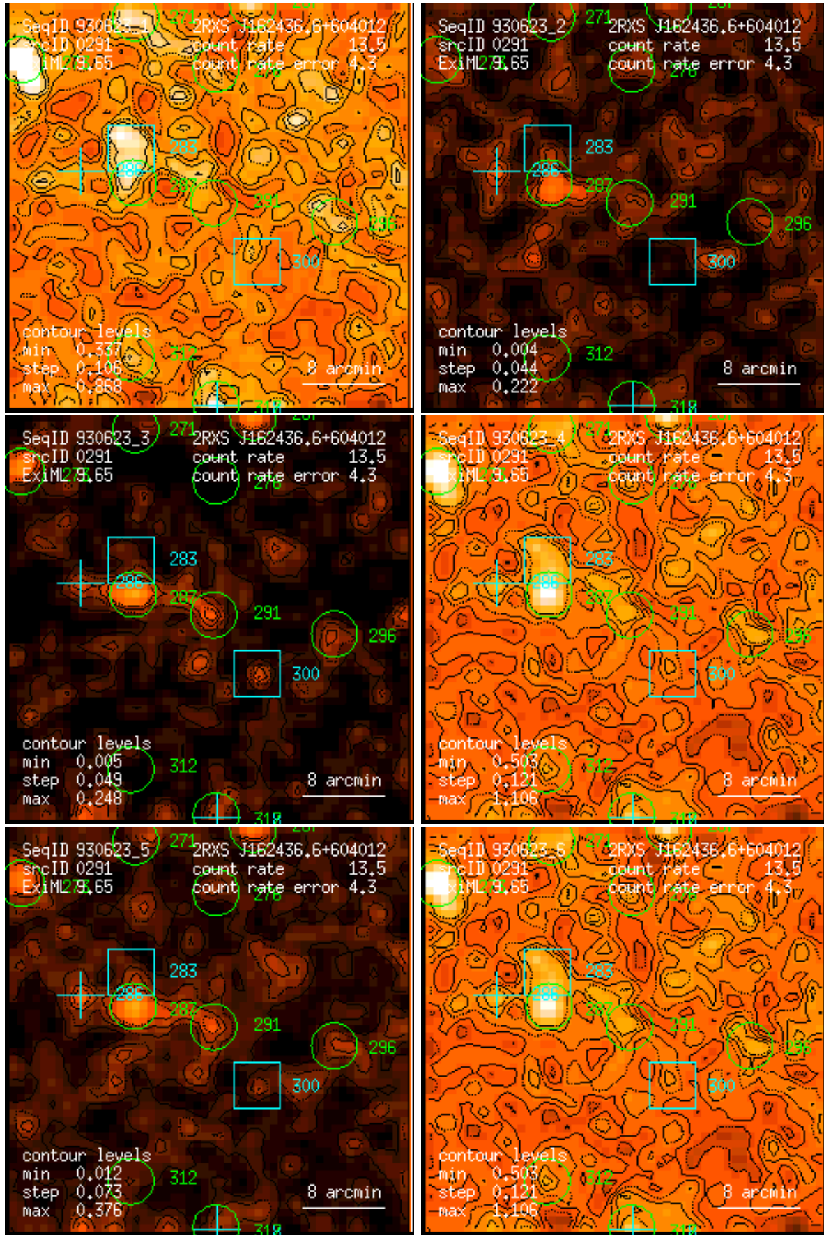
Figure 291: RASS 930623: detection 0291: band rate images, Gaussian filter: (1) PSPC channels 11 – 41, (2) 52 – 90, (3) 91 – 201, (4) 11 – 235, (5) 52 – 201, (6) 11 – 201. Broad band rates in counts/ks. Band rate contour levels in counts/ks/arcmin 2 .
